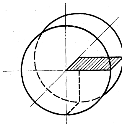
FIGURE 2 — Sample from bar or billet with a diameter or length of side > 25 \text{ mm} and \leq 40 \text{ mm}
