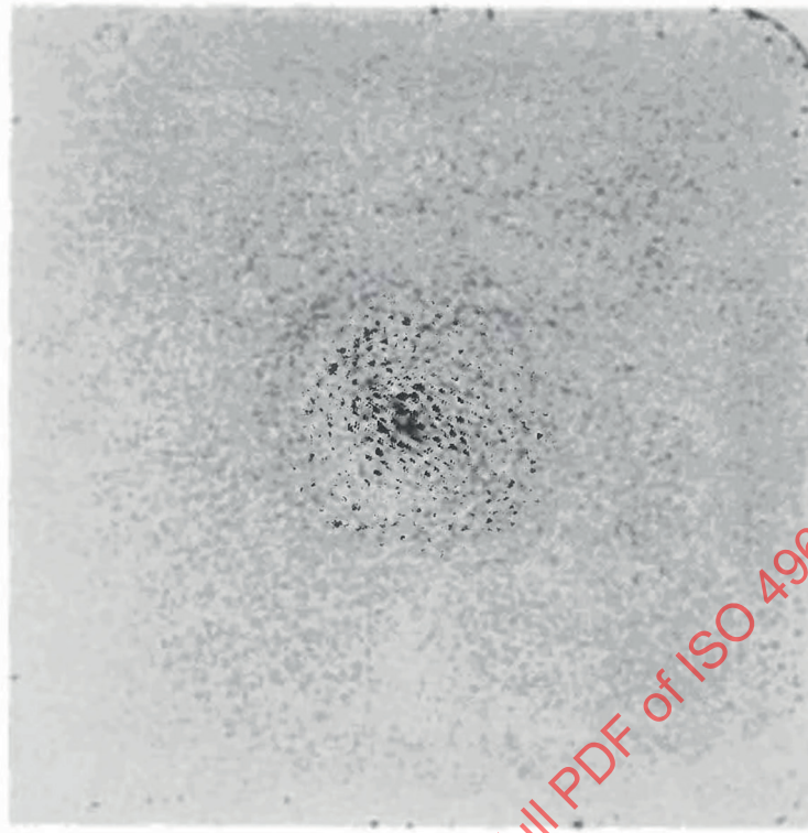
Figure A.3 — Central segregation
