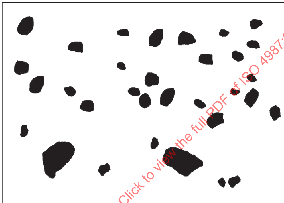
a) Maximum size allowed for a non-relevant indication for severity level SP 5
