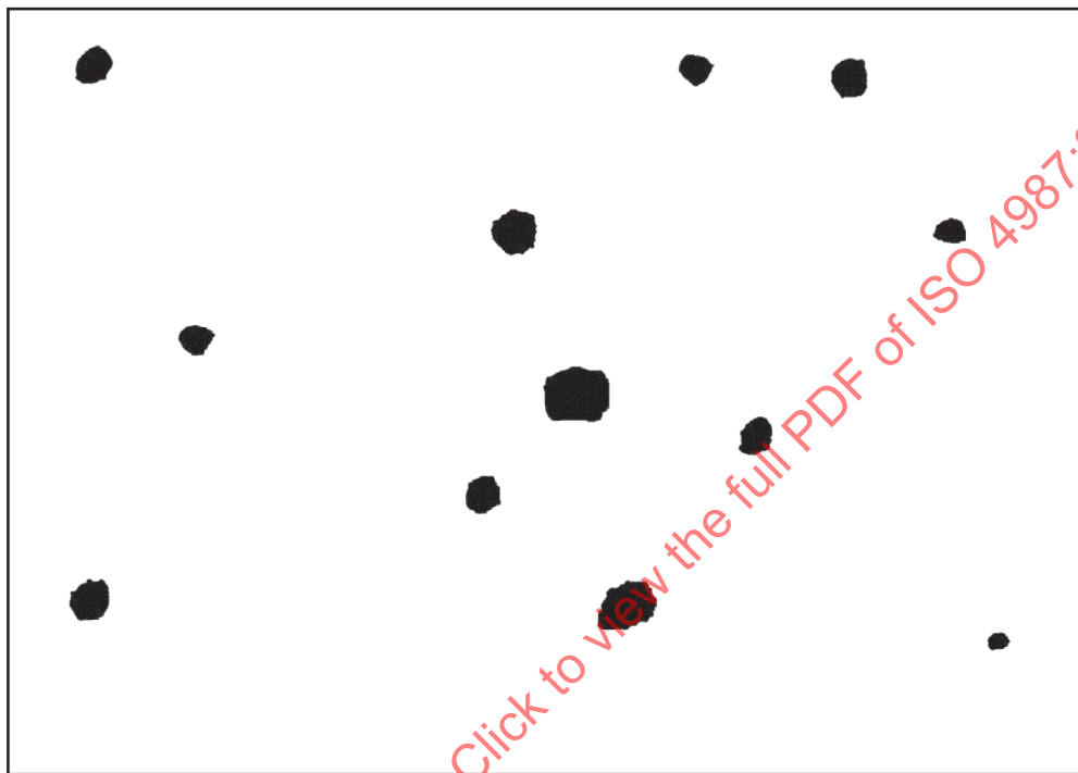
a) Maximum size allowed for a non-relevant indication for severity level SP 3
