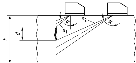
a) Wall section with broken discontinuity
