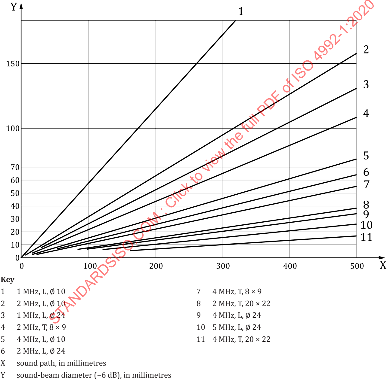
Figure A.1 — Sound-beam diameters according to sound path and near-field length for various probes
