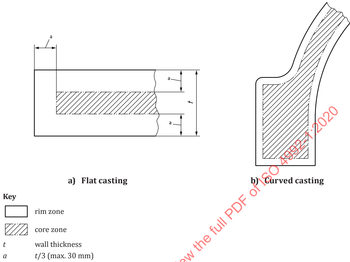
Figure 2 — Division of wall section into zones
