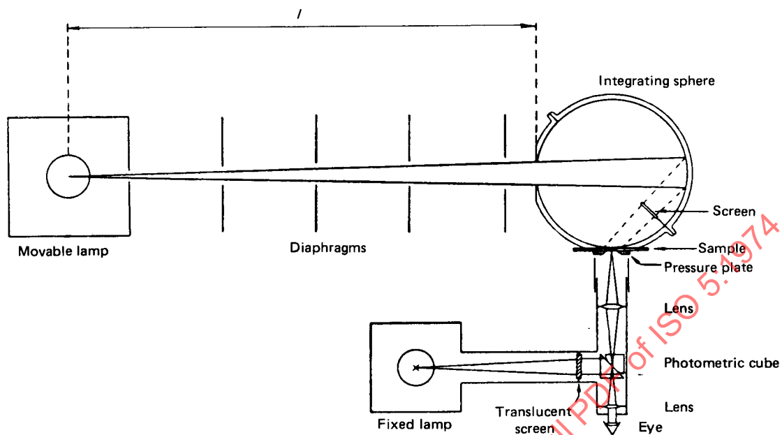
FIGURE 1 – Apparatus for integrating sphere method using inverse square law
