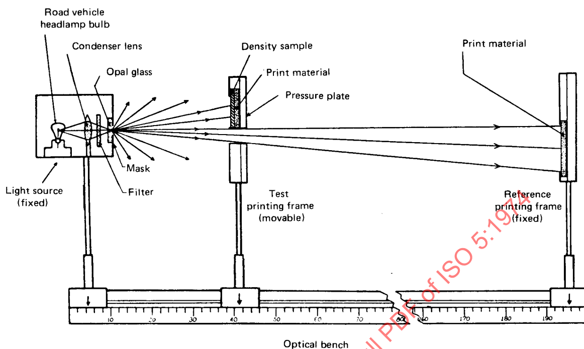
FIGURE 6 — Apparatus for contact printing method
