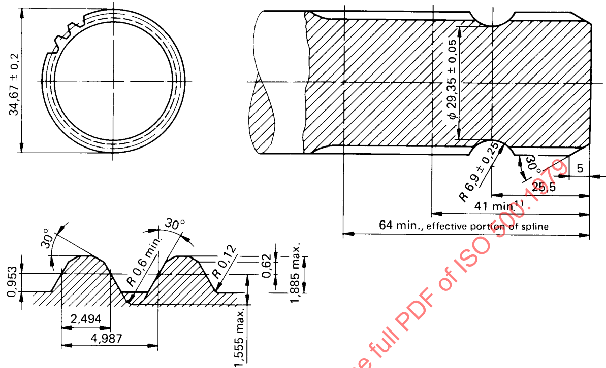
Basic profiles of shaft
