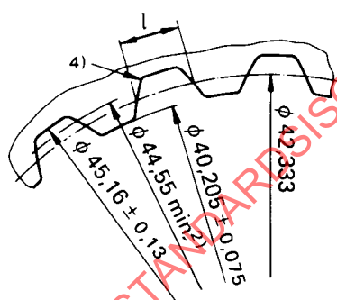
Hub profile
