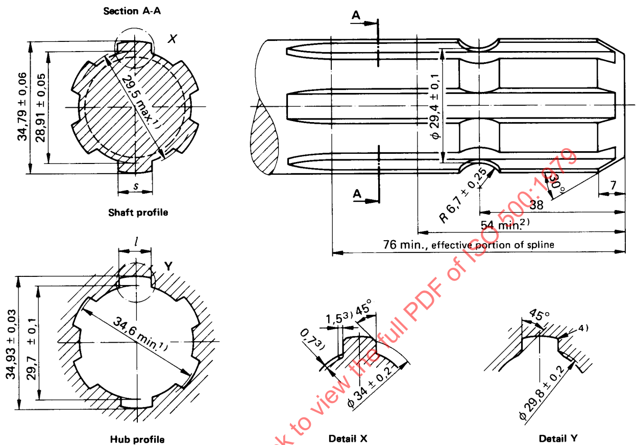
FIGURE 1 – PTO, Type 1
