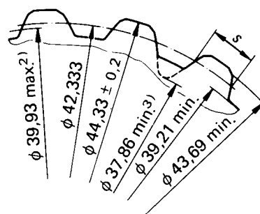
Shaft profile
