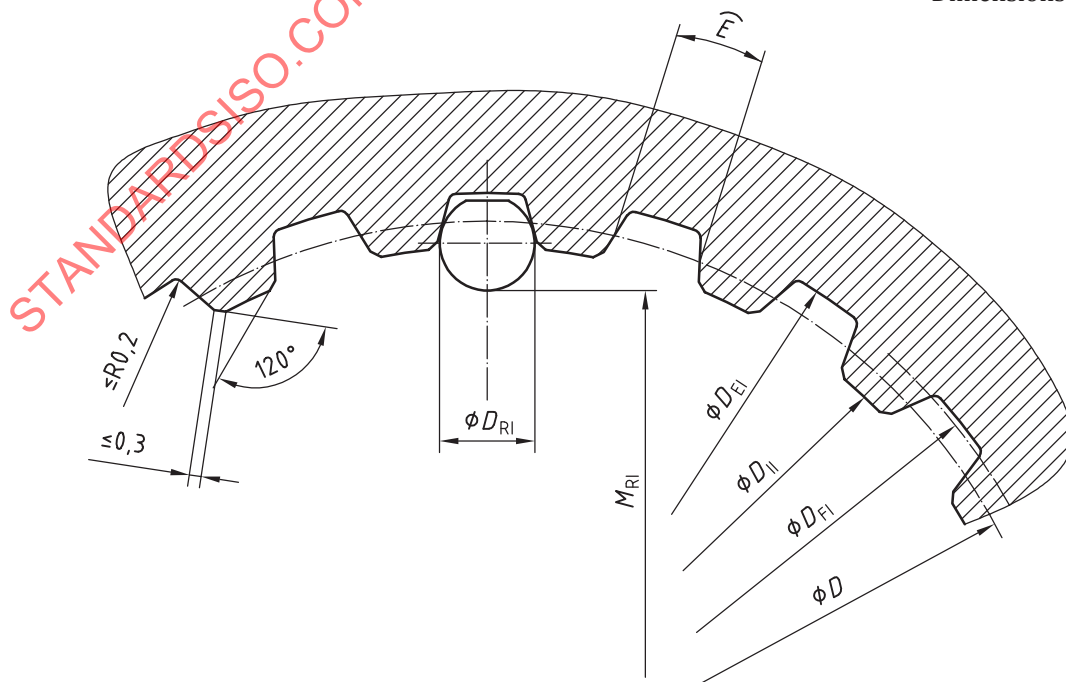
Figure 8 — Internal involute spline dimensions — Type 3
