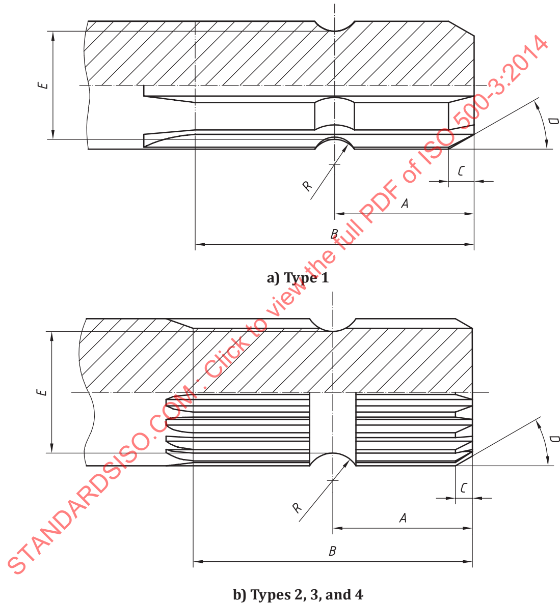
Figure 2 — PTO dimensions
