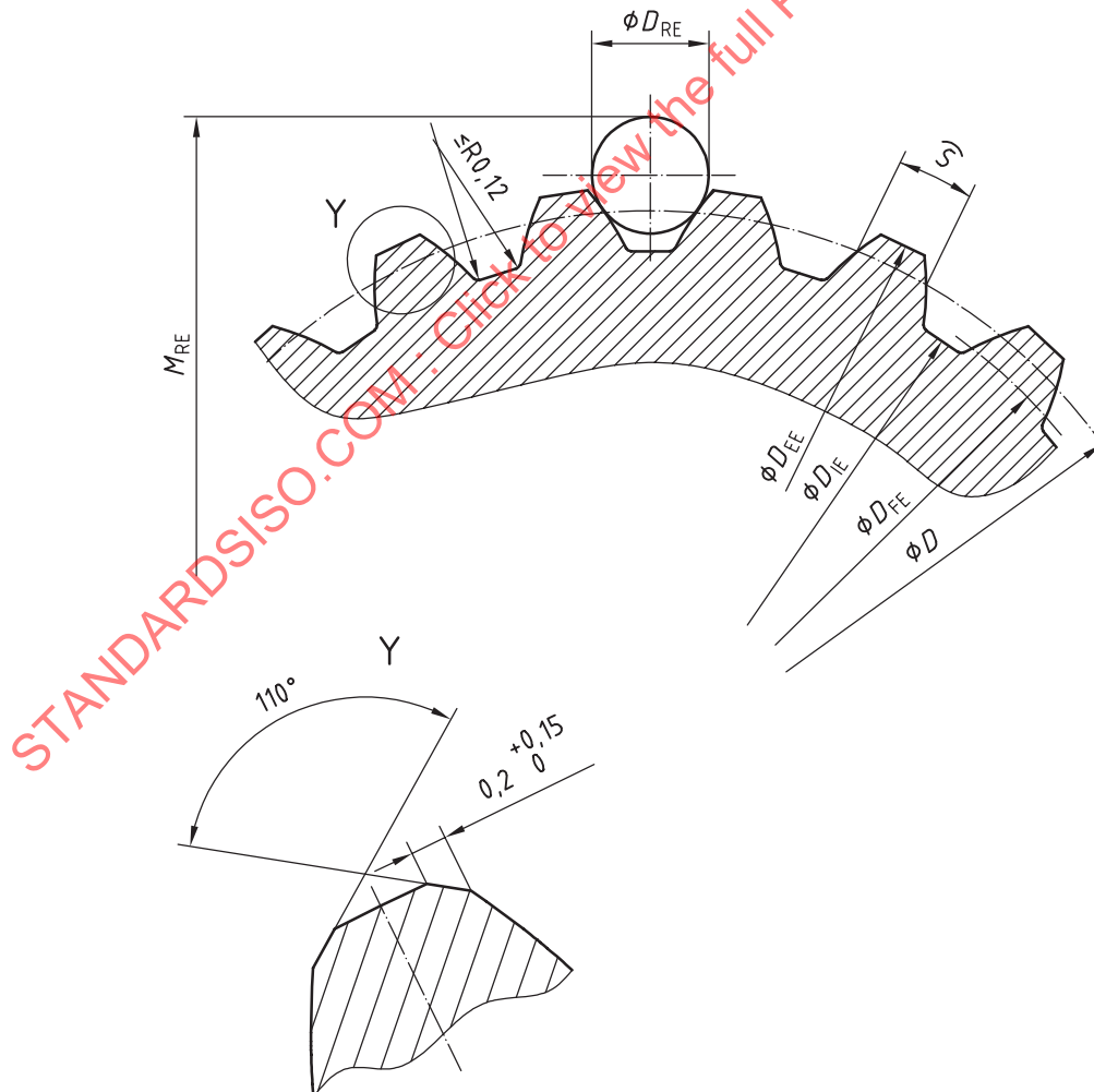
Figure 5 — External, involute spline dimensions — Type 2
