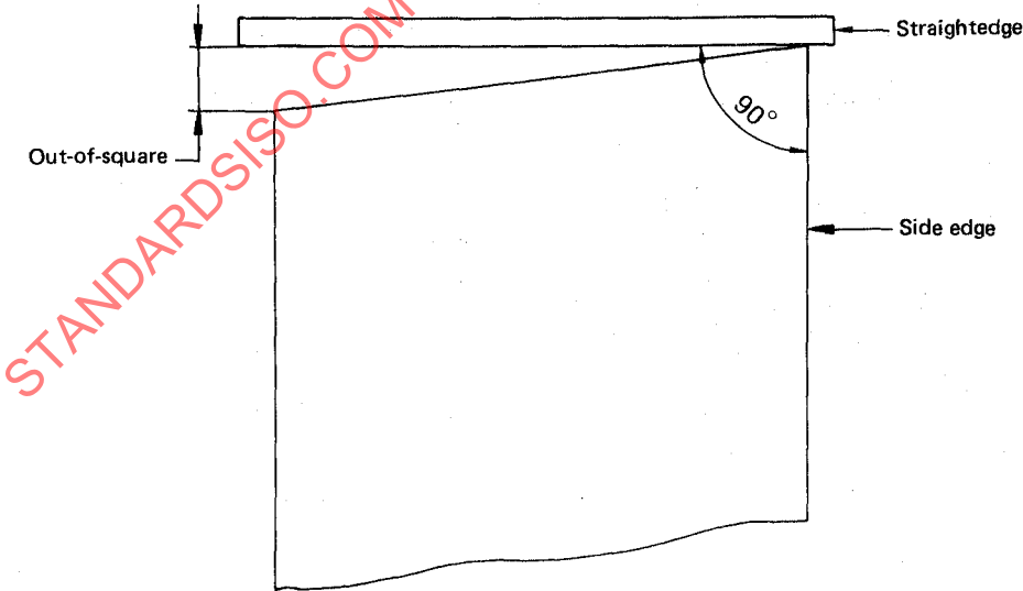
Figure 3 — Measurement of out-of-square
