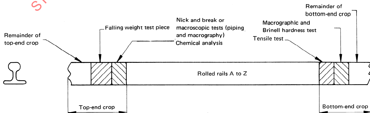
Figure 1 — Location of samples
