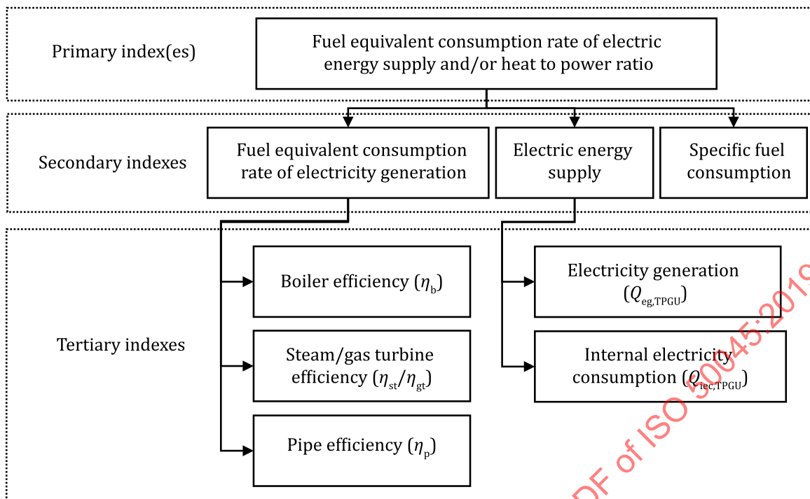
Figure 2 — Index structure of evaluation of energy savings for a TPGU
