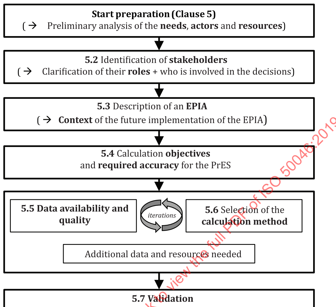
Figure 4 — Overview of the preparation process
