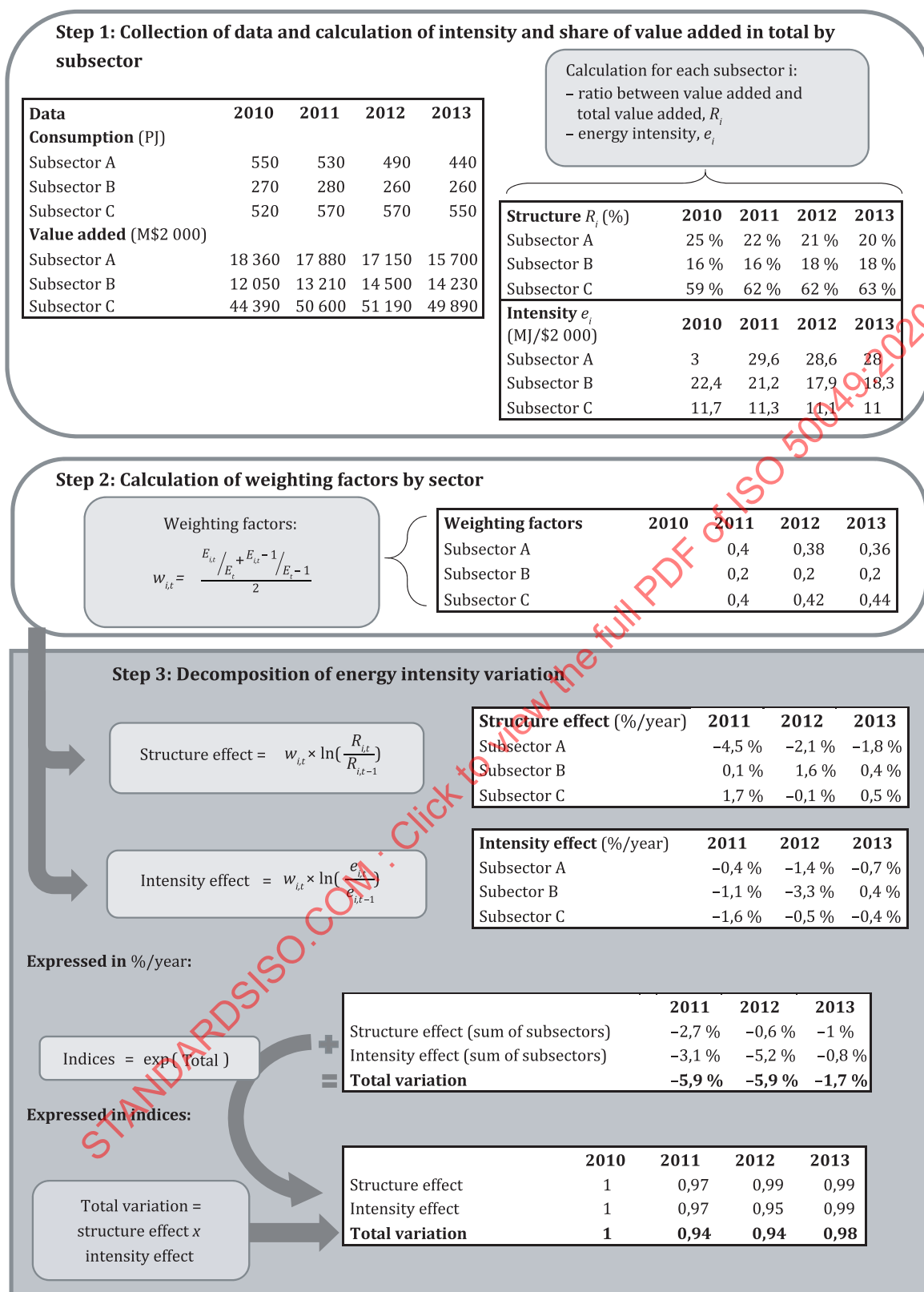
Figure A.3 — Calculation of structure effect with the AMDI Divisia method
