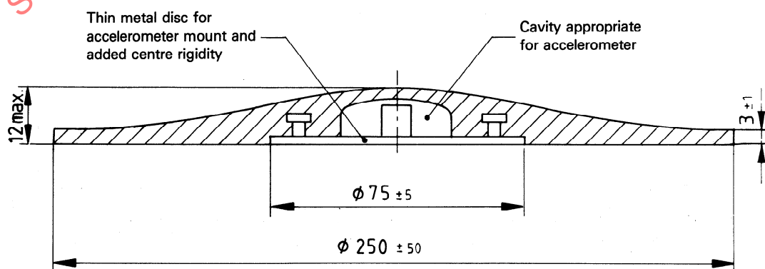
Figure 3 — Design for semi-rigid disc
