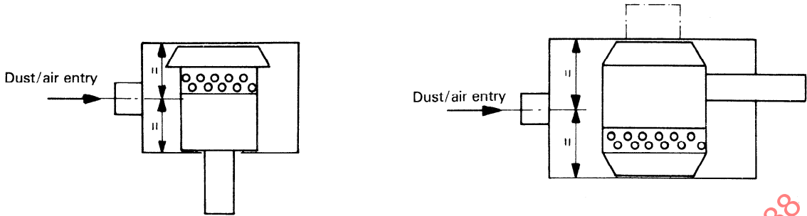
Figure 13 — Non-tubular inlet air cleaner test chamber arrangement
