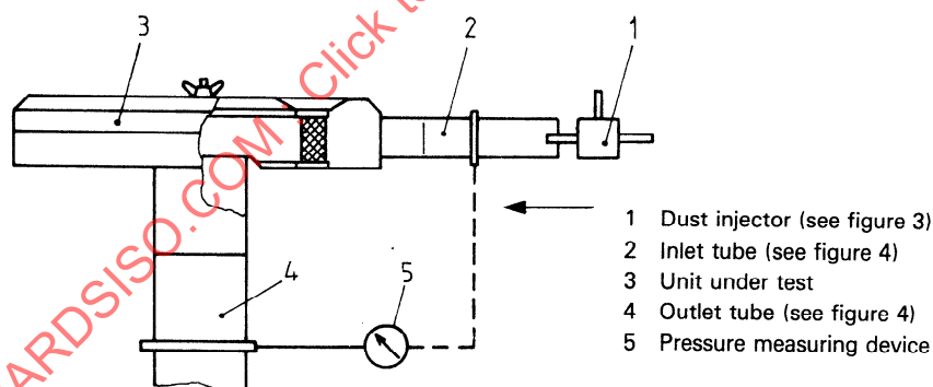
Figure 11 — Assembly efficiency/capacity test set-up
