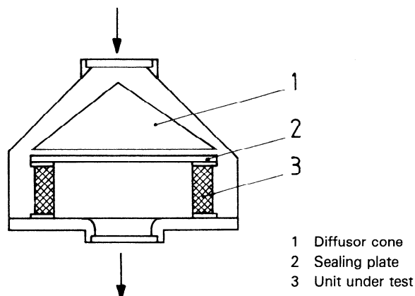
Figure 5 — Filter element test shroud
