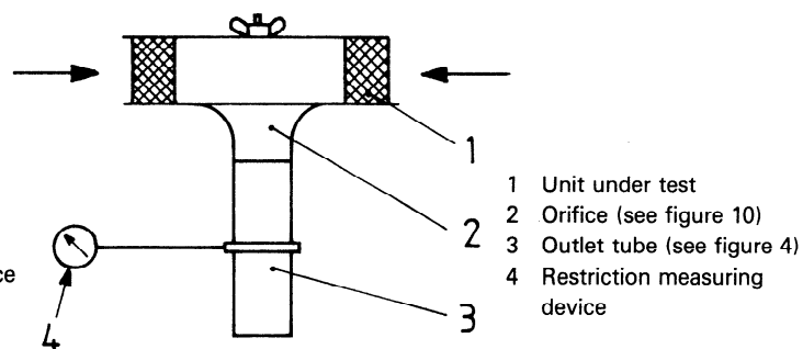
Figure 9 — Filter element restriction test set-up
