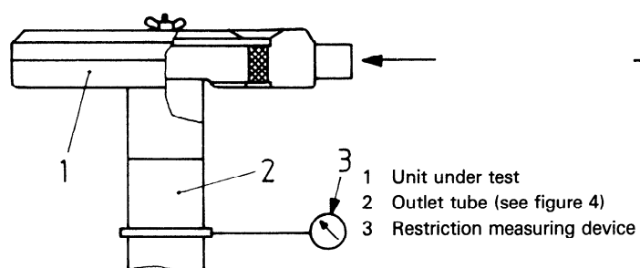
Figure 8 — Assembly restriction test set-up
