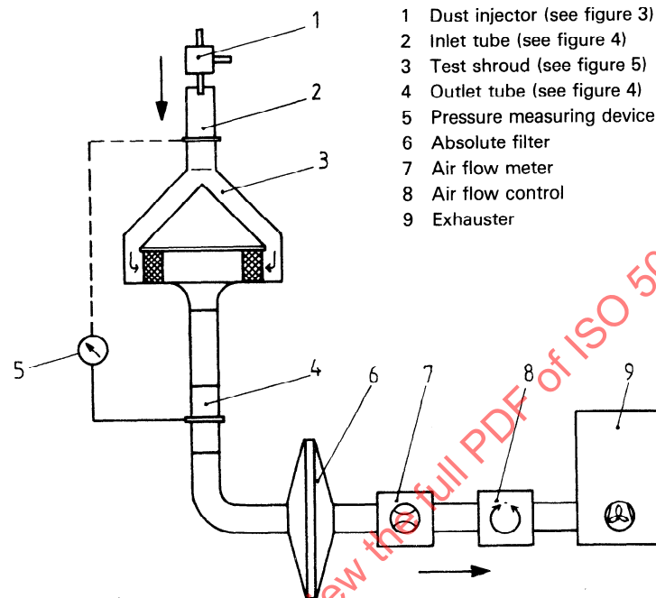
Figure 2 — Filter element efficiency/capacity test set-up
