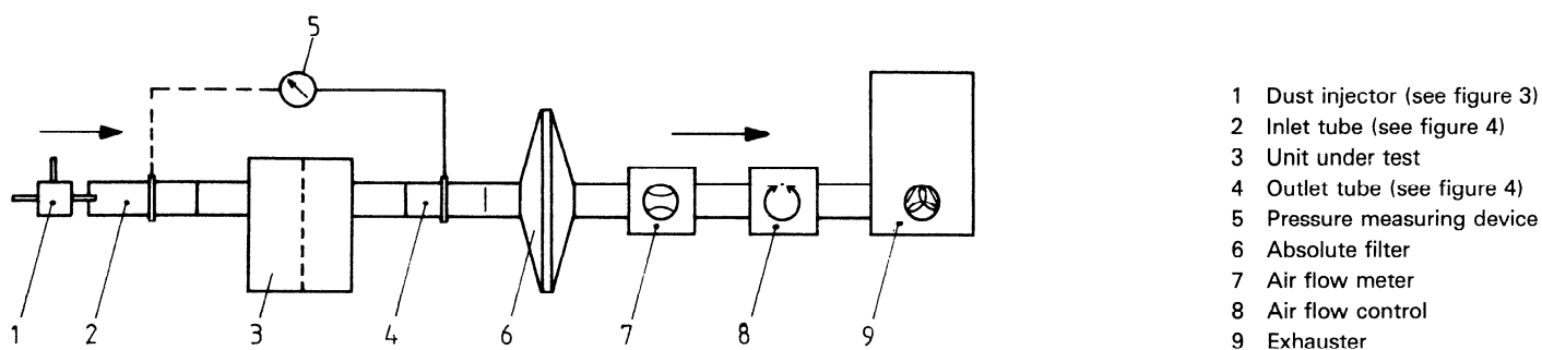
Figure 12 — Tubular inlet air cleaner efficiency/capacity test set-up
