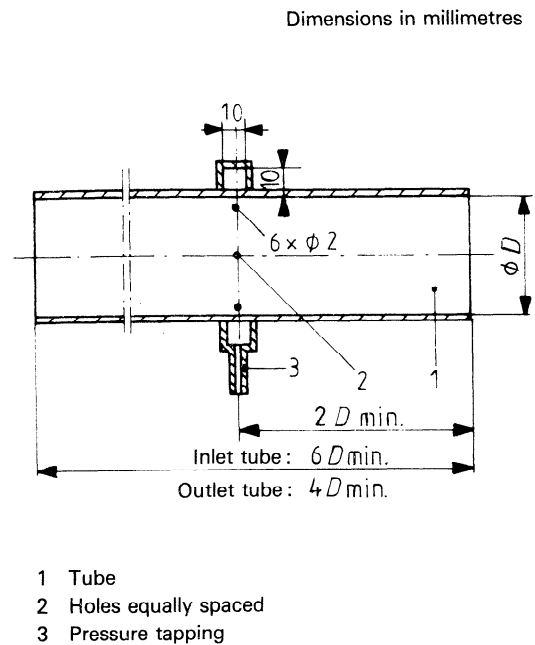
Figure 4 — Inlet outlet piezometer tube
