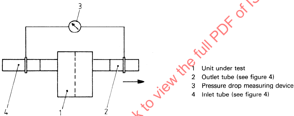
Figure 14 — Assembly pressure drop test set-up
