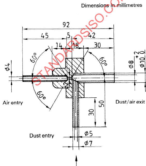
Figure 3 — Dust injector
