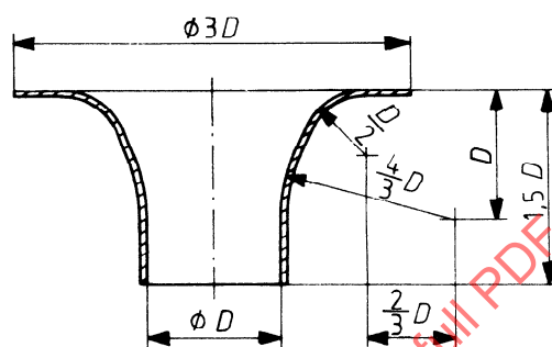
Figure 10 — Ideal flow orifice
