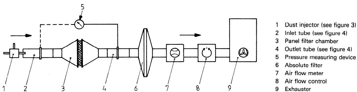
Figure 7 — Panel filter element efficiency/capacity test set-up
