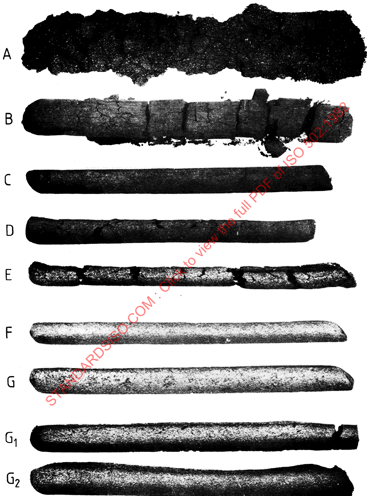
Figure 1 — Gray-King coke type
