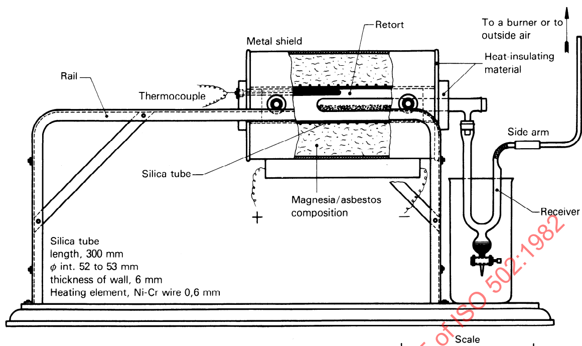
Figure 2 — Single tube furnace
