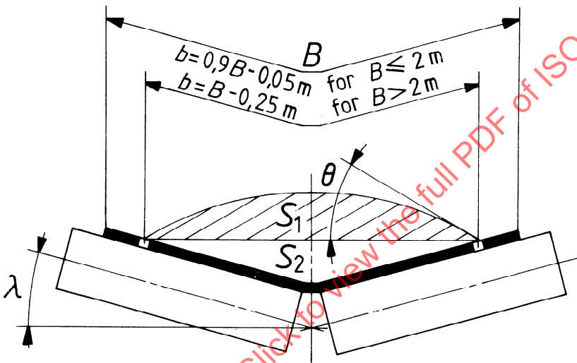
b) With two carrying idlers
