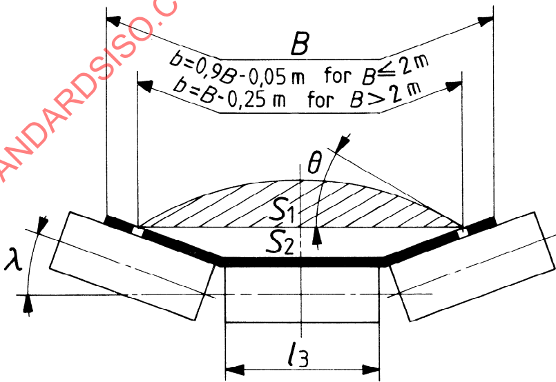
c) With three carrying idlers
