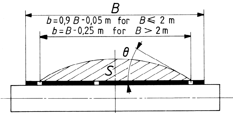
a) With one carrying idler
