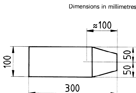
Figure 3 — Tapered test piece
