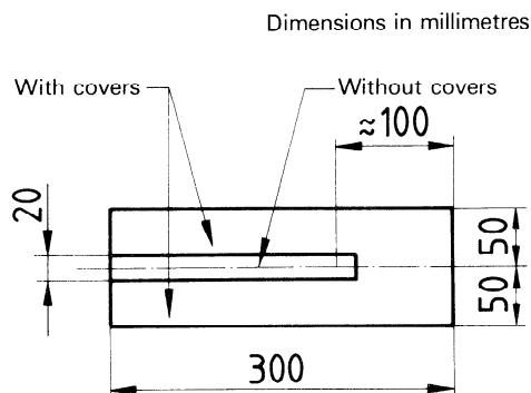
Figure 1 — Test piece with breaker
