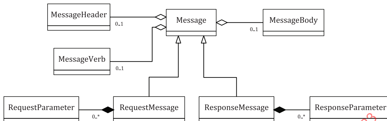
Figure 1 — Abstract message architecture
