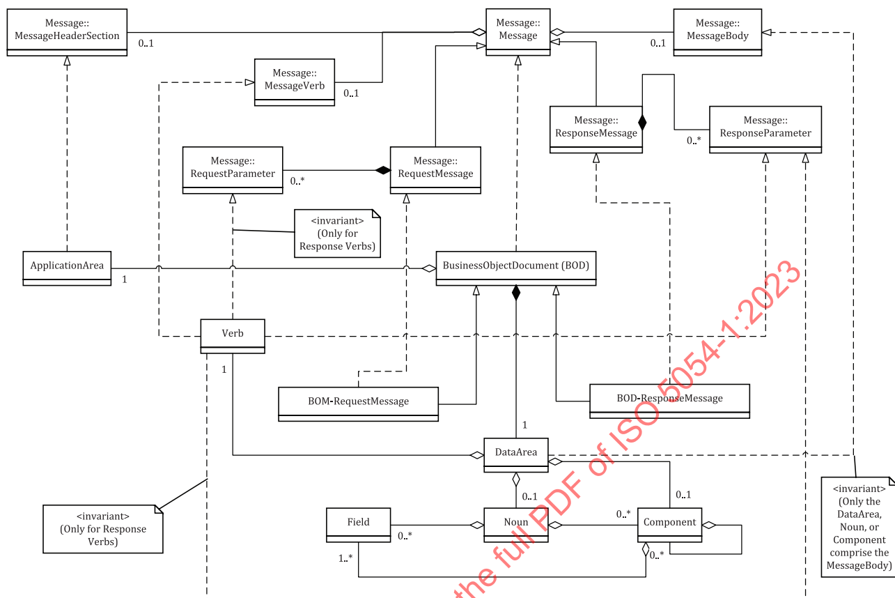
Figure 2 — BOD message architecture
