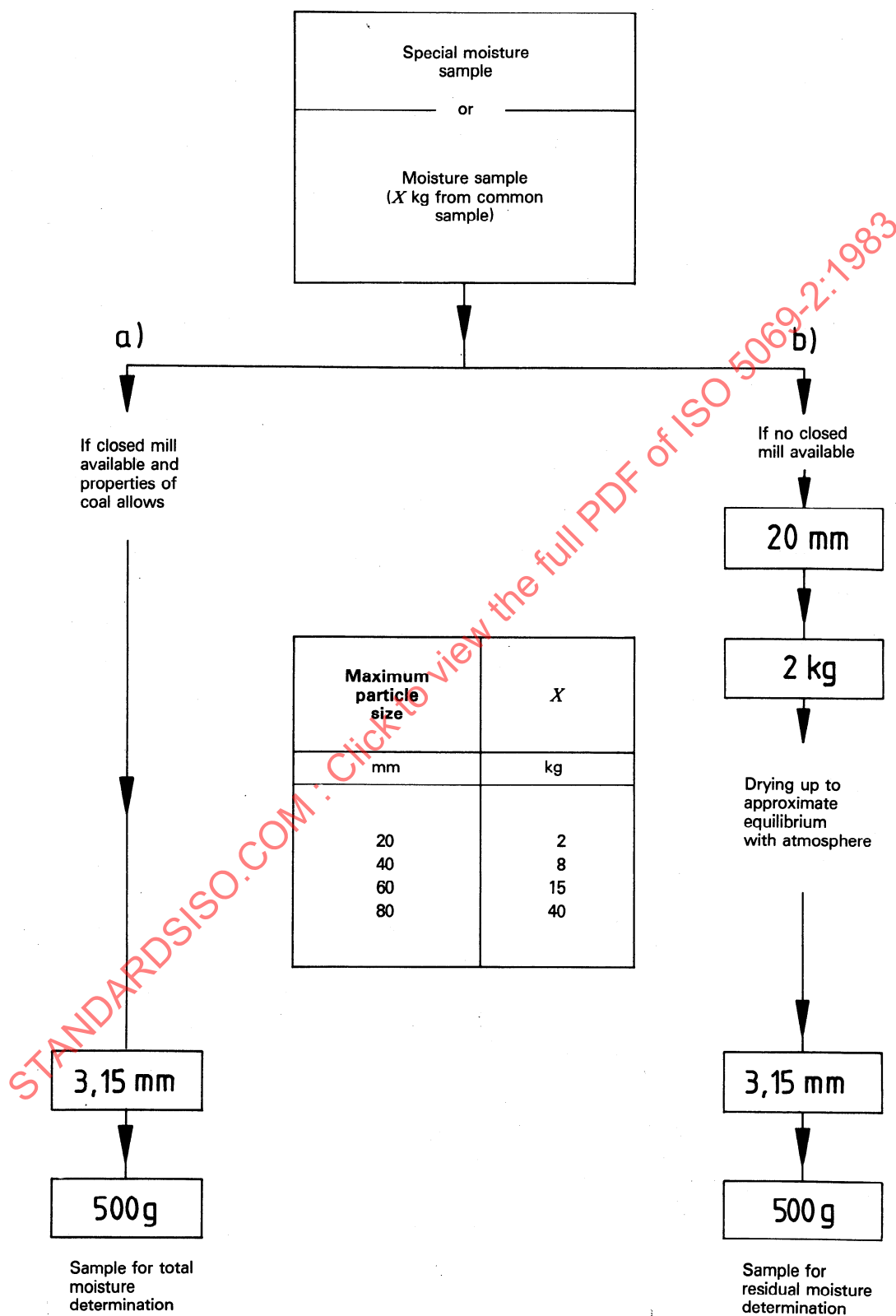
Figure 2 — Sample preparation for moisture determination
