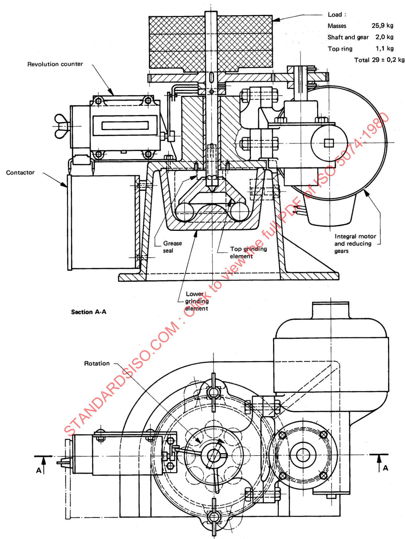
Figure 1 — Hardgrove grindability machine
