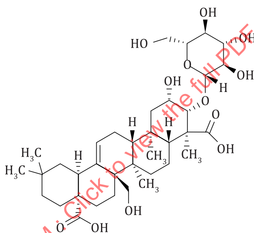
Figure B.1 — Chemical structures of tenuifolin
