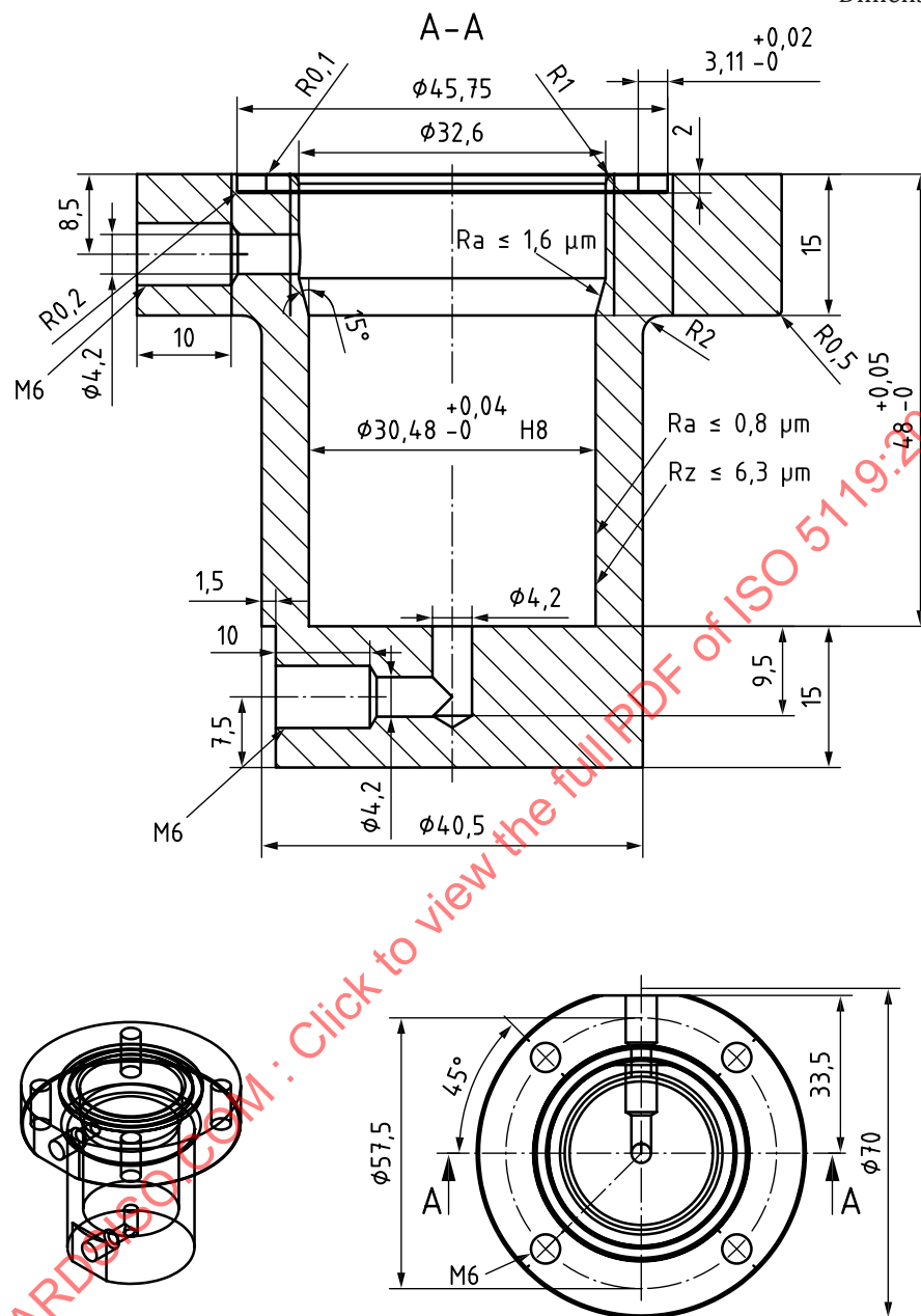
Figure A.2 — Isometric, cross-section and top view of female fixture
