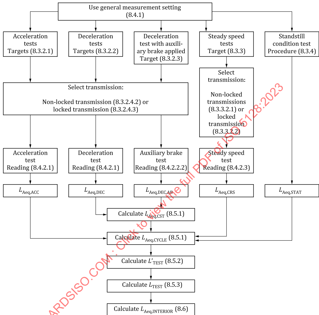
Figure B.2 — Flowchart for vehicles with auxiliary brake
