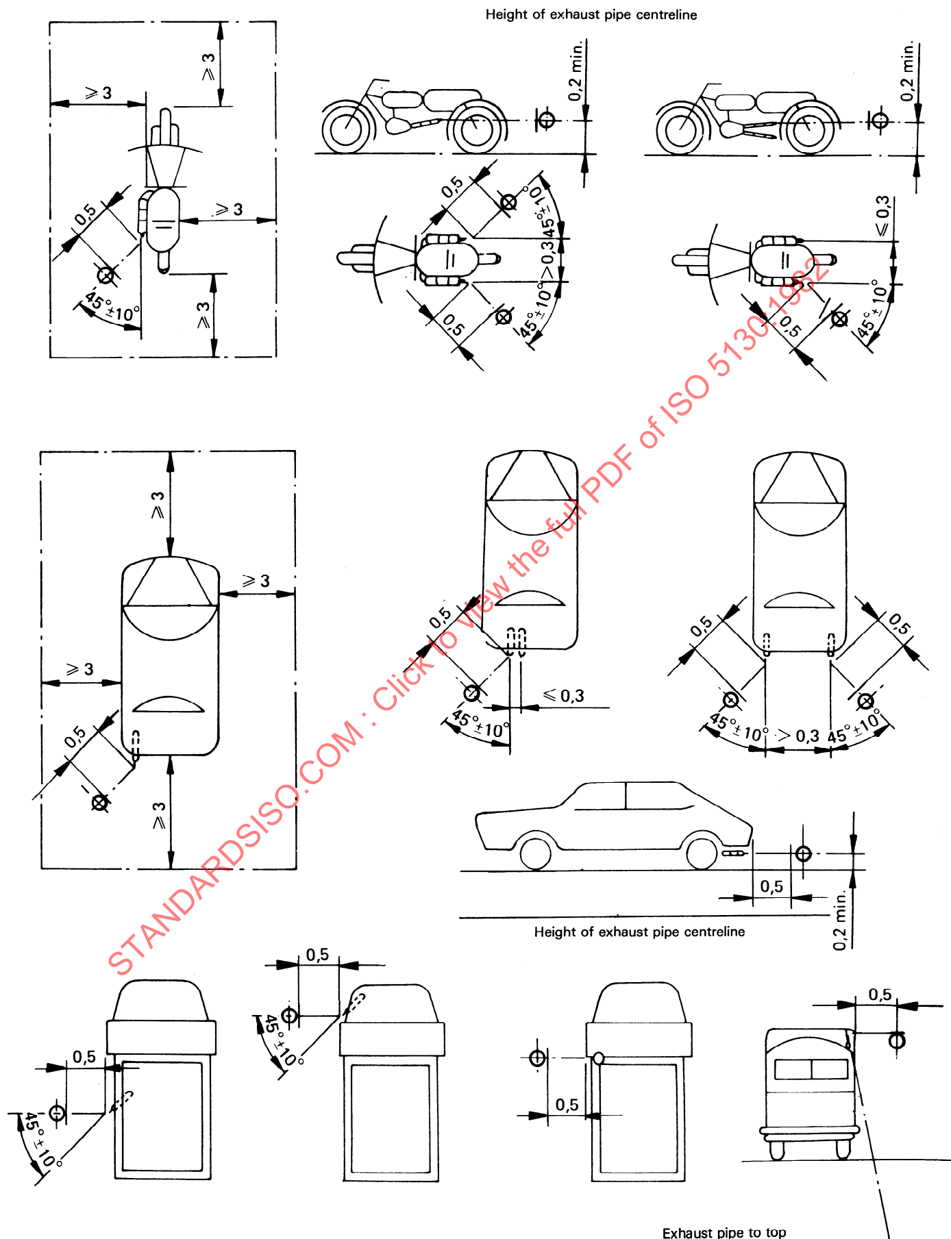
Figure 1 — Test site and microphone positions for measuring exhaust noise
