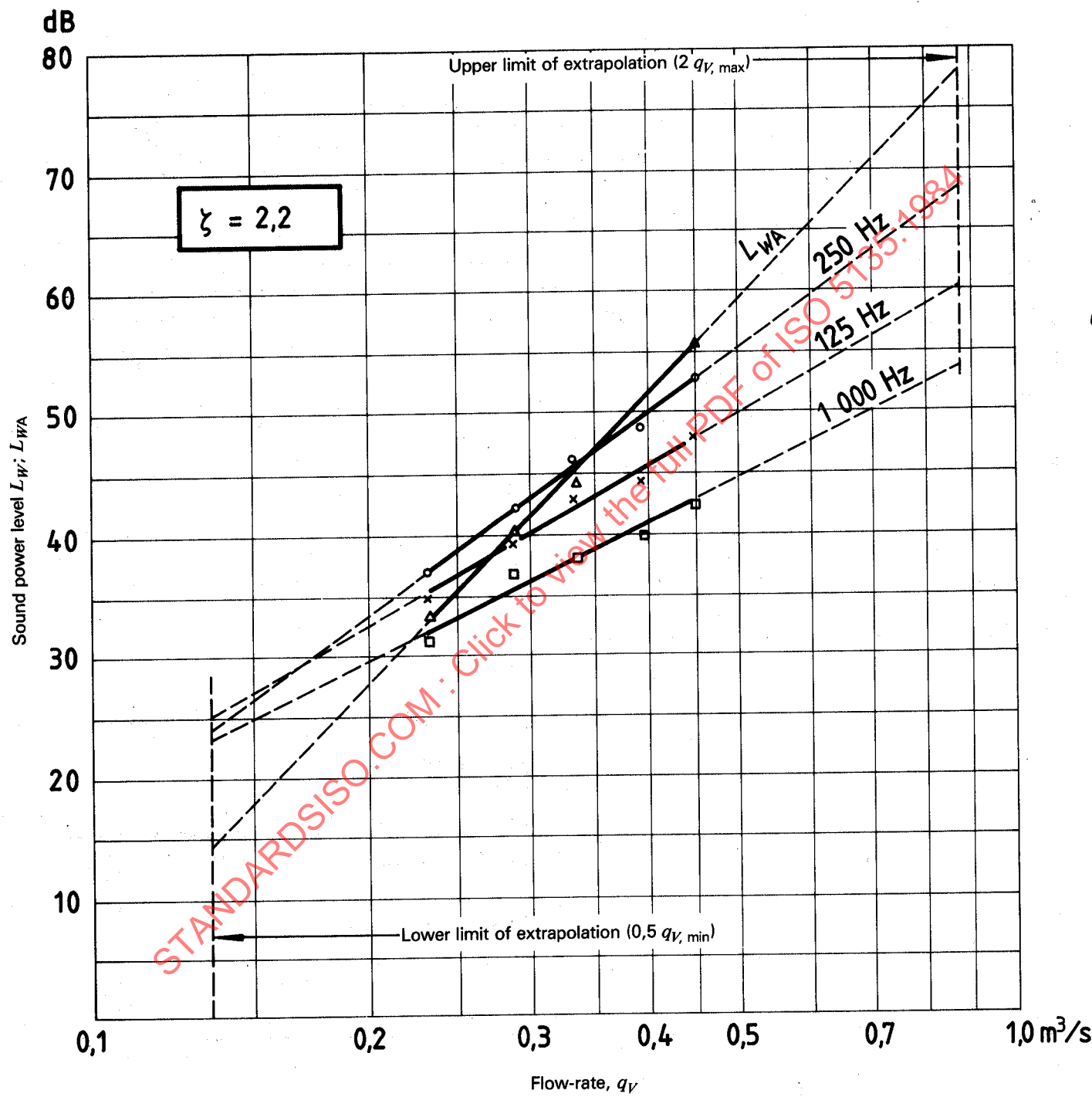
Figure 7 a) — Examples of L_W and L_{WA} plotted against \lg q_V for an assembly with constant total pressure loss coefficient
