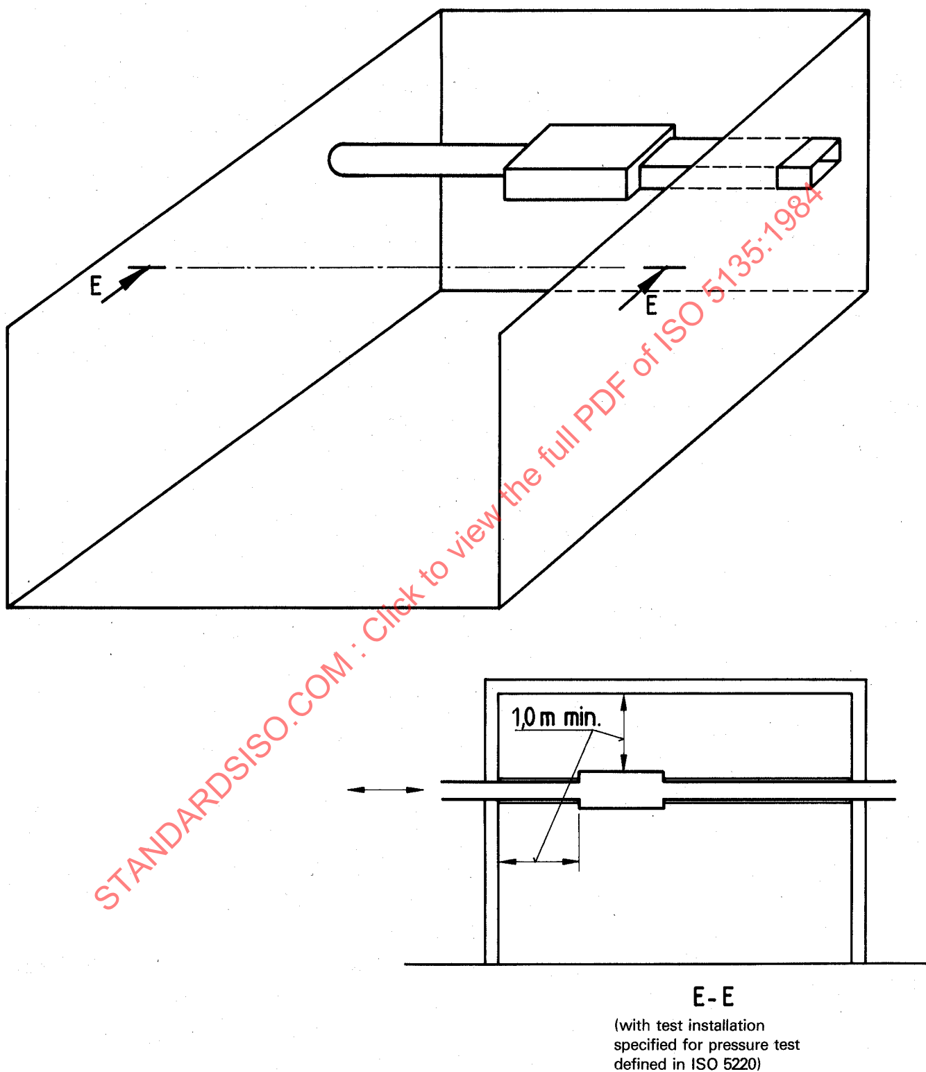
Figure 6 — Mounting detail for air control device to determine casing radiated sound
