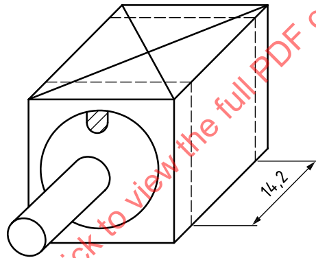
Figure A.2 — Cutting of test specimens in the longitudinal (length) direction
