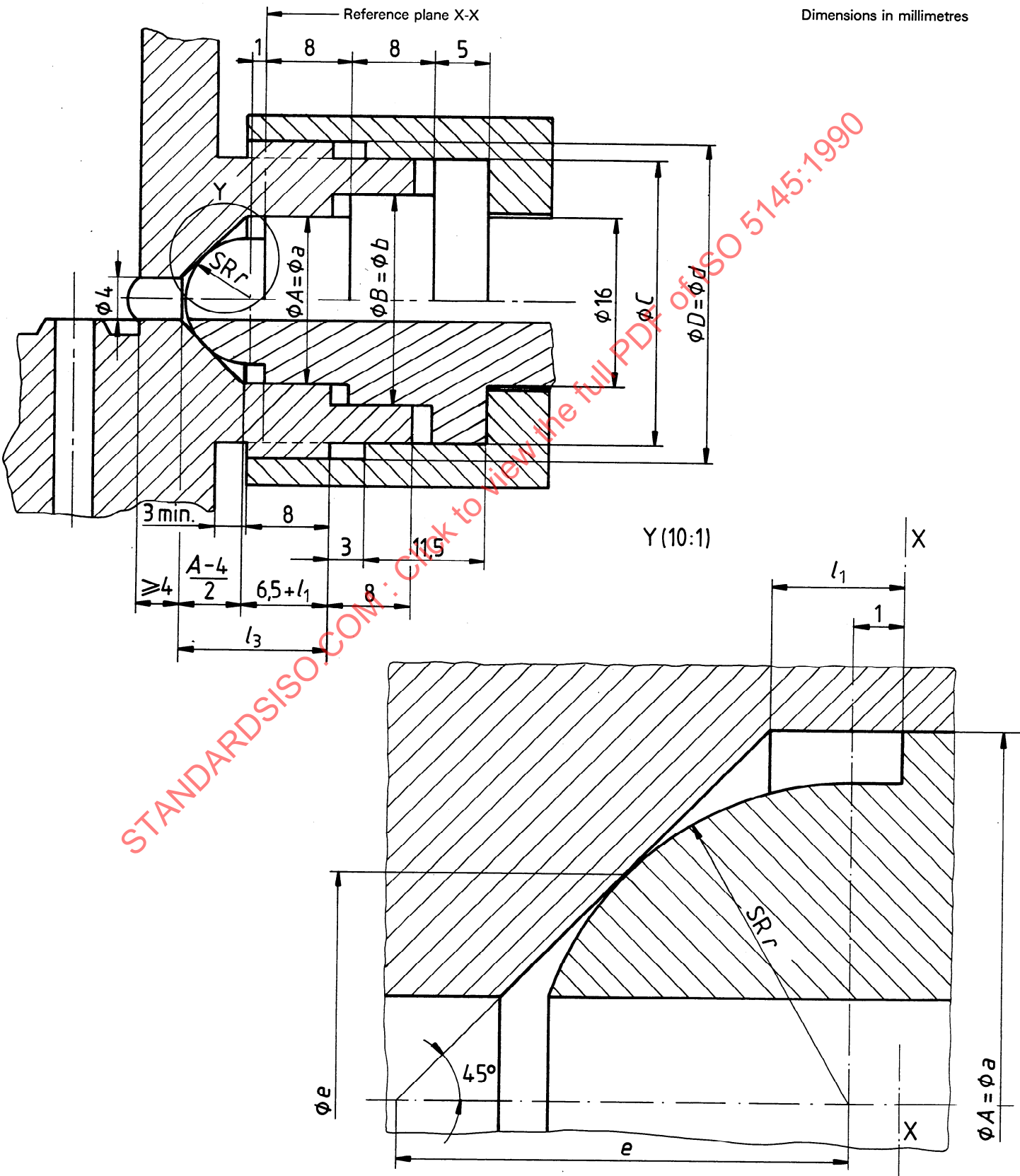
Figure C.1 — Bull-nose connector
