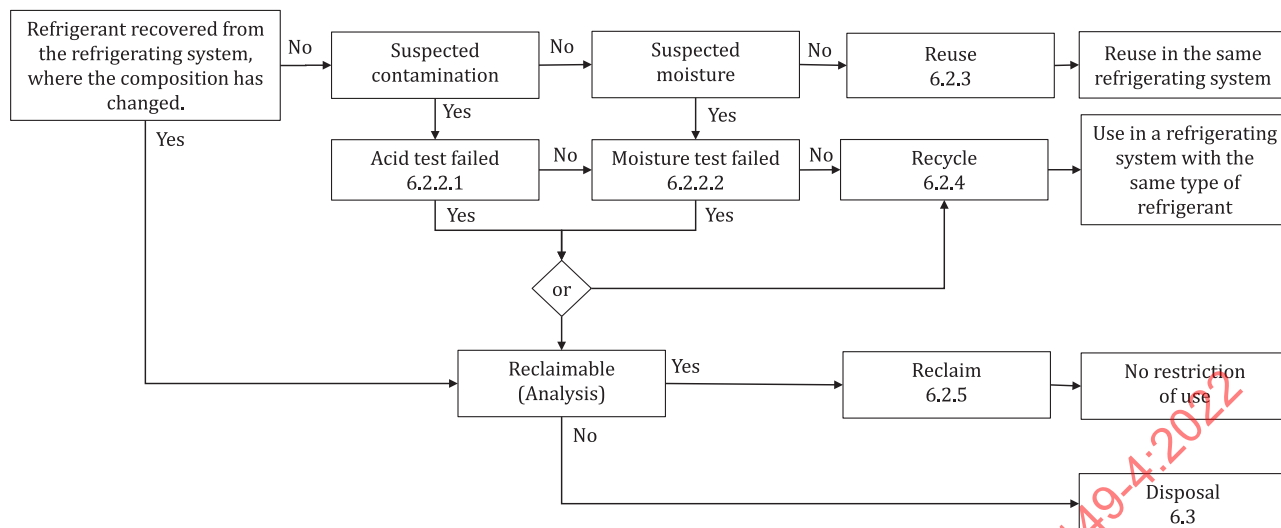
Figure 2 — Flow chart for recovered refrigerant
