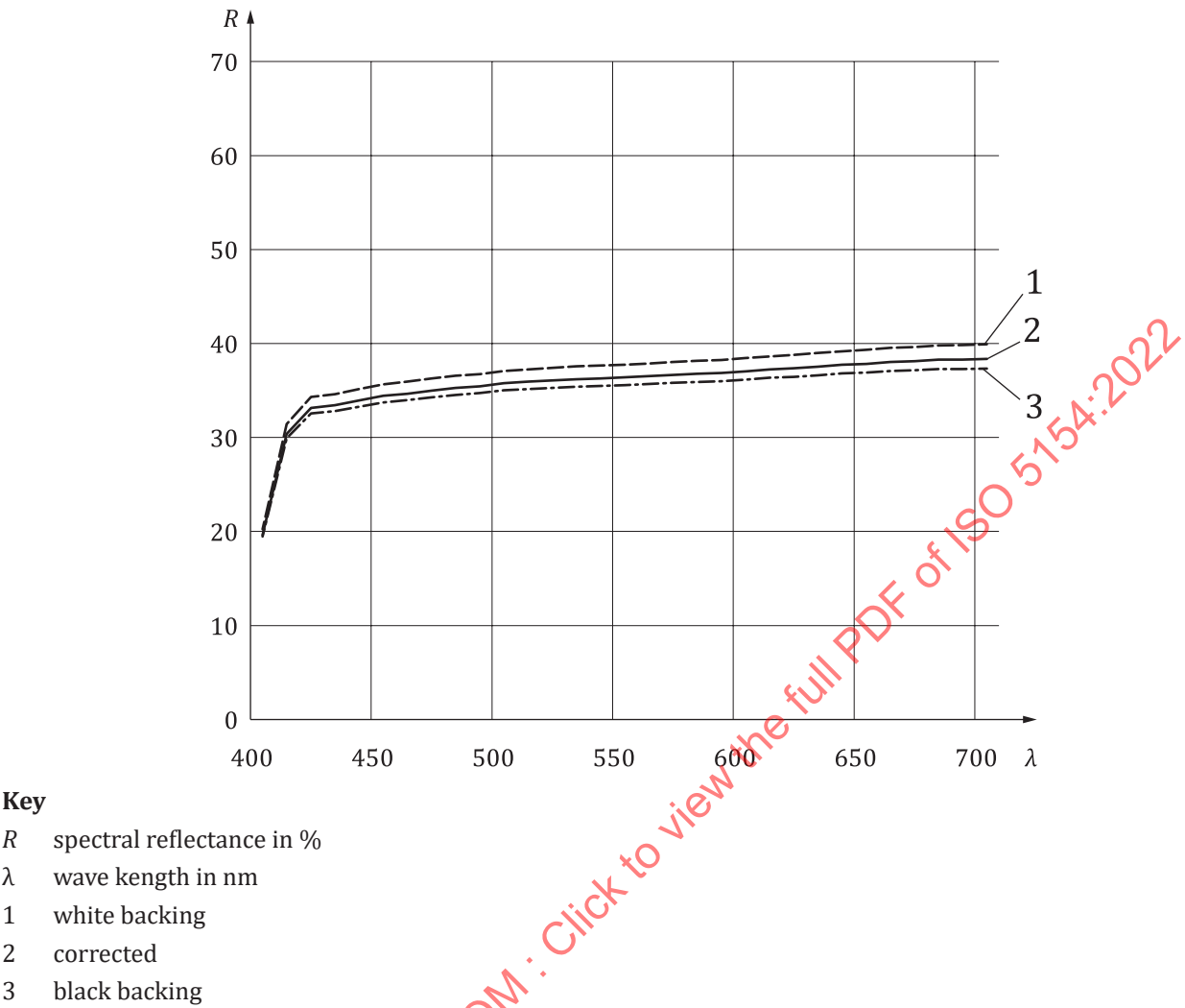
Figure B.4 — Low hiding sample spectrum reflectance measurement result
