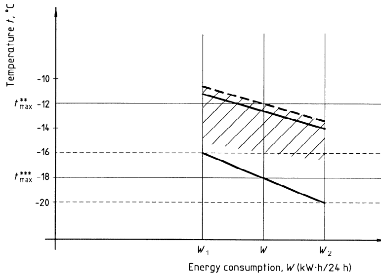
Figure 6 — Example of the determination of energy consumption by interpolation (see 15.2.2)
