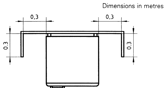
Figure 2 — Partitions to restrict air circulation (plan view)
