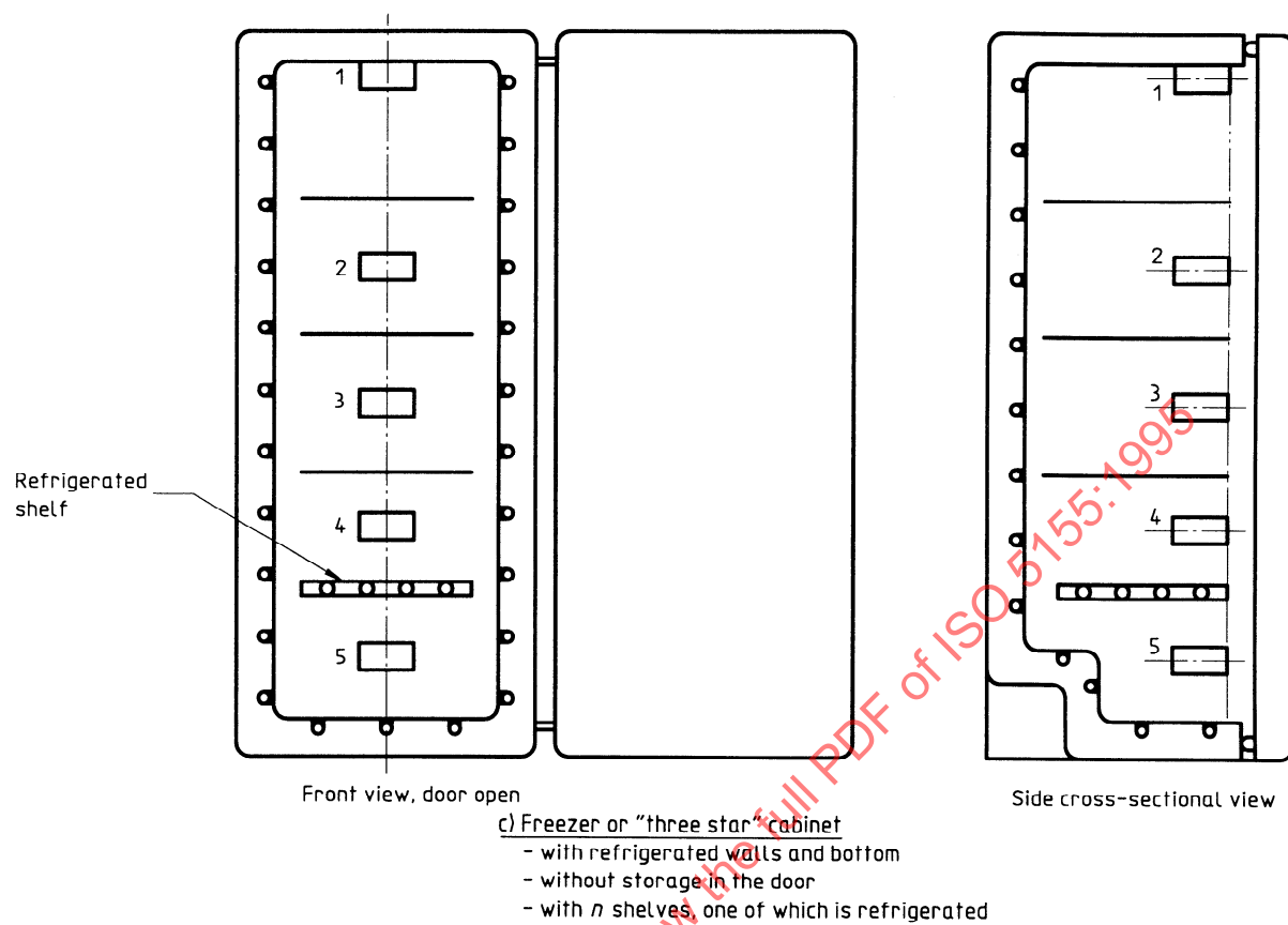
Figure 11 — Examples of positioning of "M" packages (continued)
