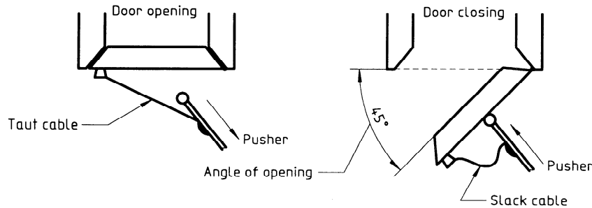
Figure 3 — Example of opening and closing of external door(s)
