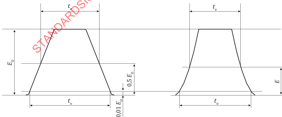
Figure A.2 — Typical shutter traces
