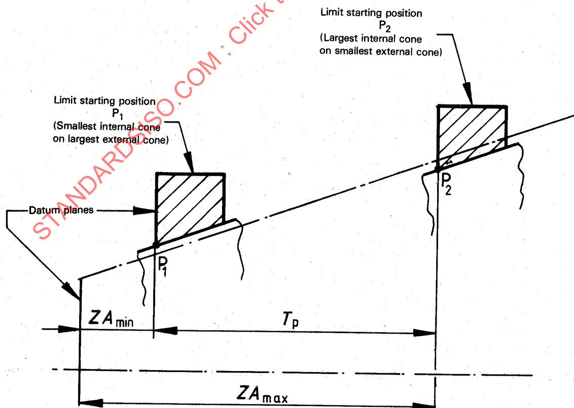
Figure 7 — Limit starting positions
