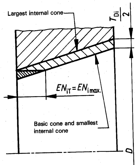
d) Internal cone — Position of deviation H
