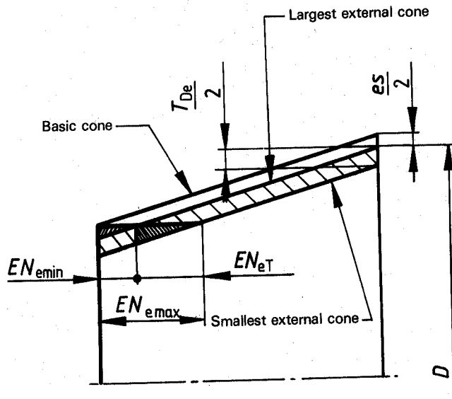
a) External cone — Positions of deviations a to g
