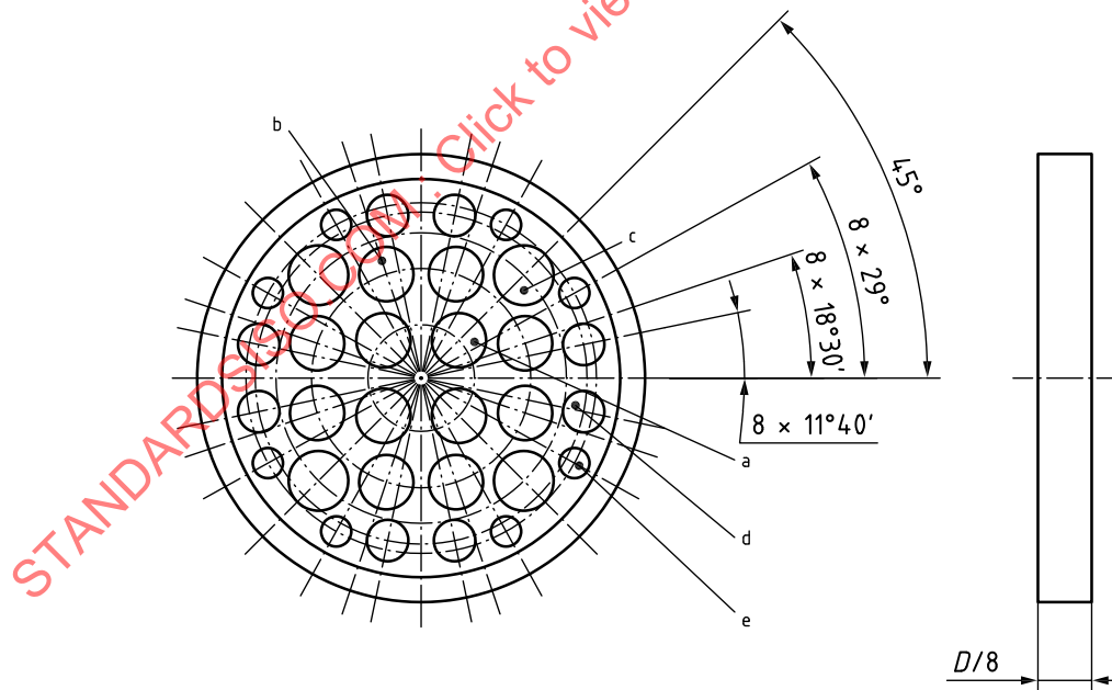
Figure 10 — Drawing of the Zanker flow conditioner plate
