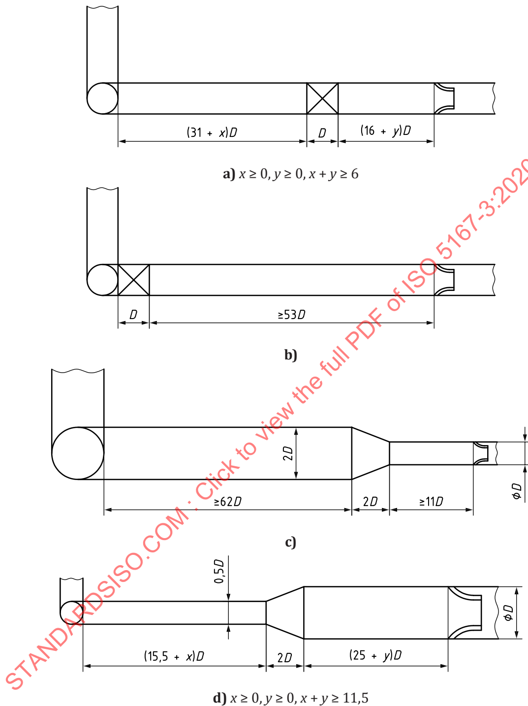
Figure 8 — Examples of acceptable installations (see 6.2.9)
