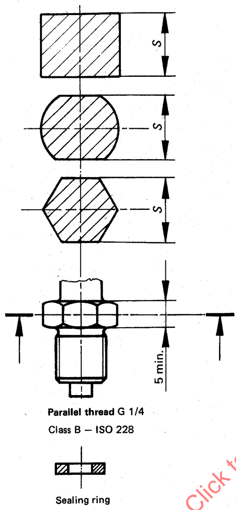
Figure 2 — Thread connection
