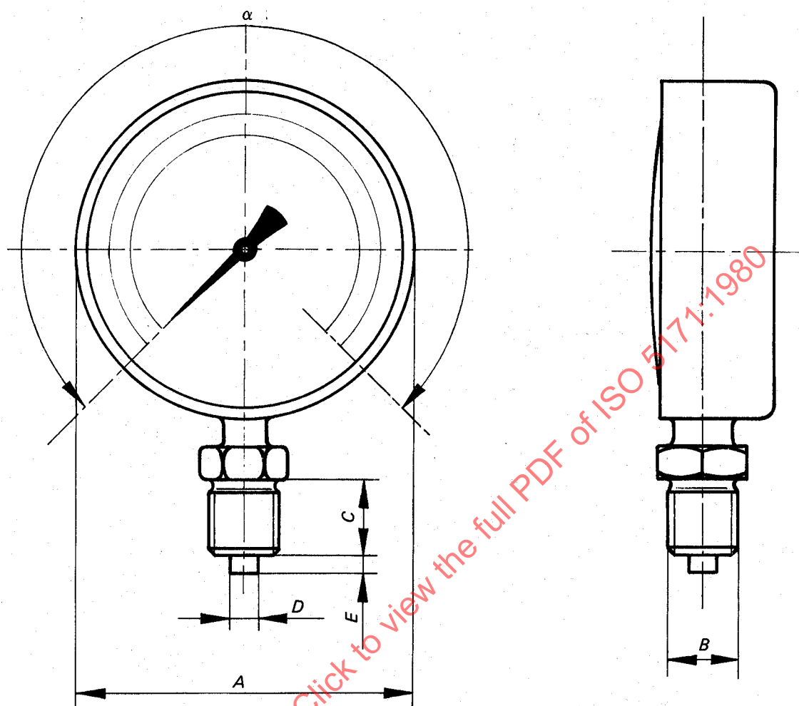
Figure 1 — Pressure gauge
