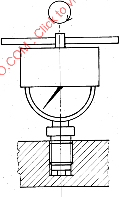
Figure 5 — Torsion test
