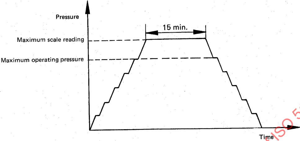
Figure 4 — Accuracy test
