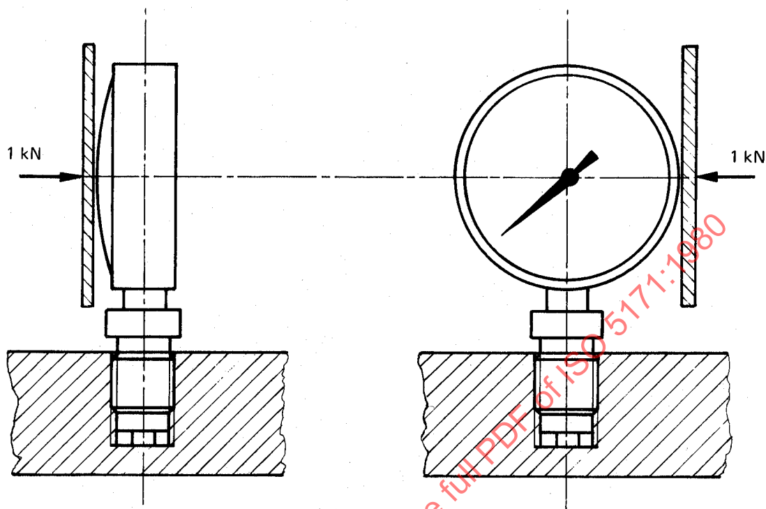
Figure 6 — Bend test
