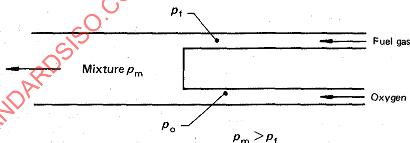
FIGURE 1 — High-pressure blowpipe
