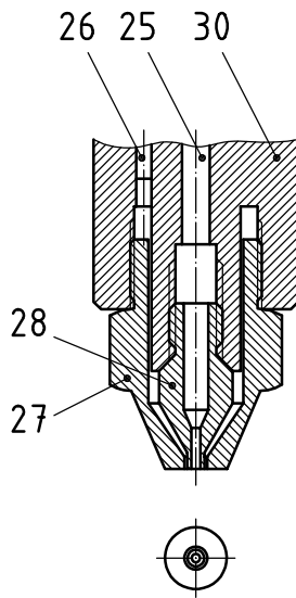
Figure B.10 — Ring-type nozzle (premixing)
