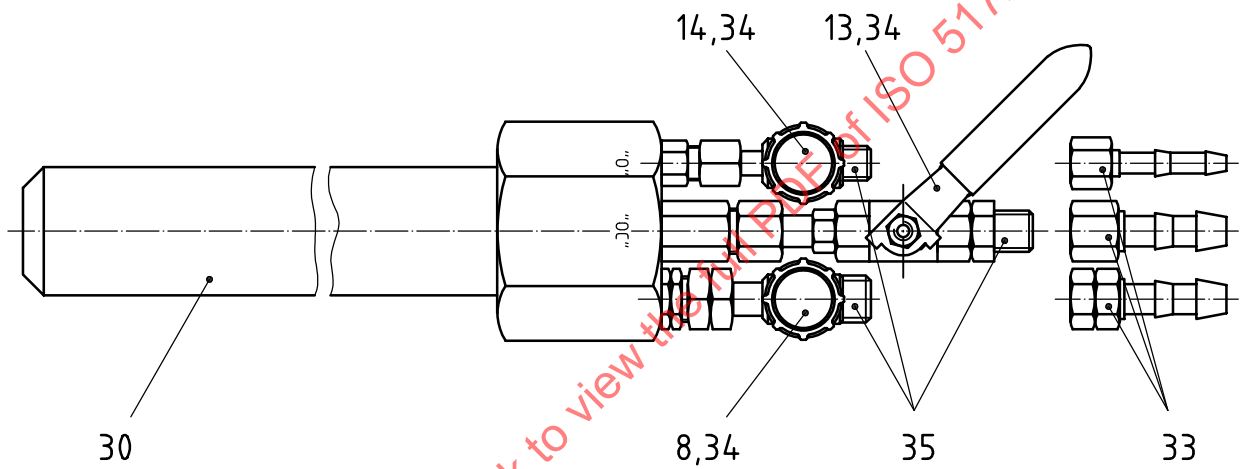
b) Machine cutting blowpipe with pre-mixing or nozzle mixing (3-hose blowpipe)
