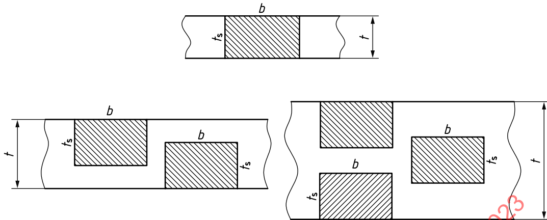
Figure 9 — Root and face bend test specimens for a butt weld (TFBB, TRBB, LFBB, LRBB and FBCB)
