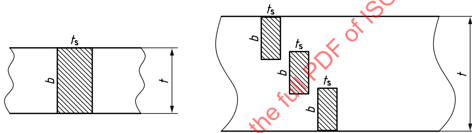
Figure 10 — Side bend test specimens for a butt weld (TSBB and SBCB)
