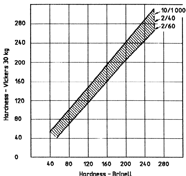
Figure B.2 — Conversion of Vickers 30 kg hardness to Brinell hardness
