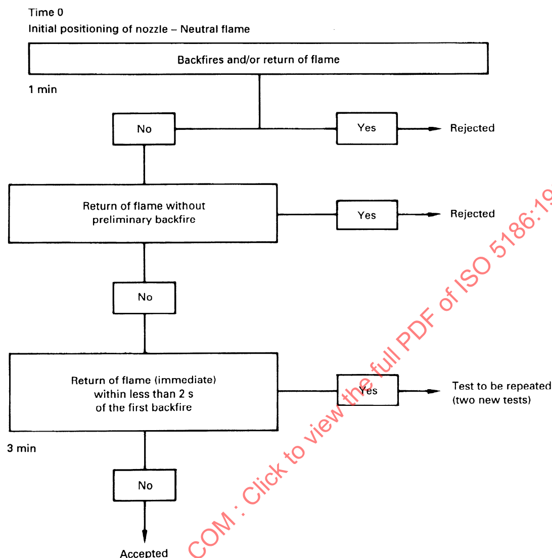
Figure 8 — Acceptance requirements
