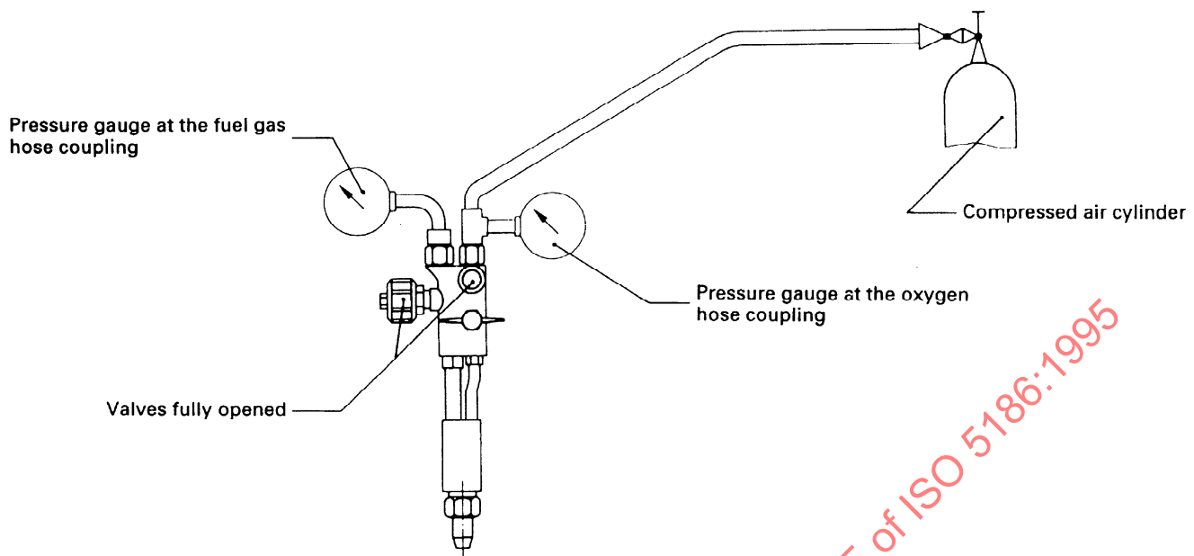
Figure 13 — Assembly for testing the resistance against backflow of heating oxygen in the fuel gas line
