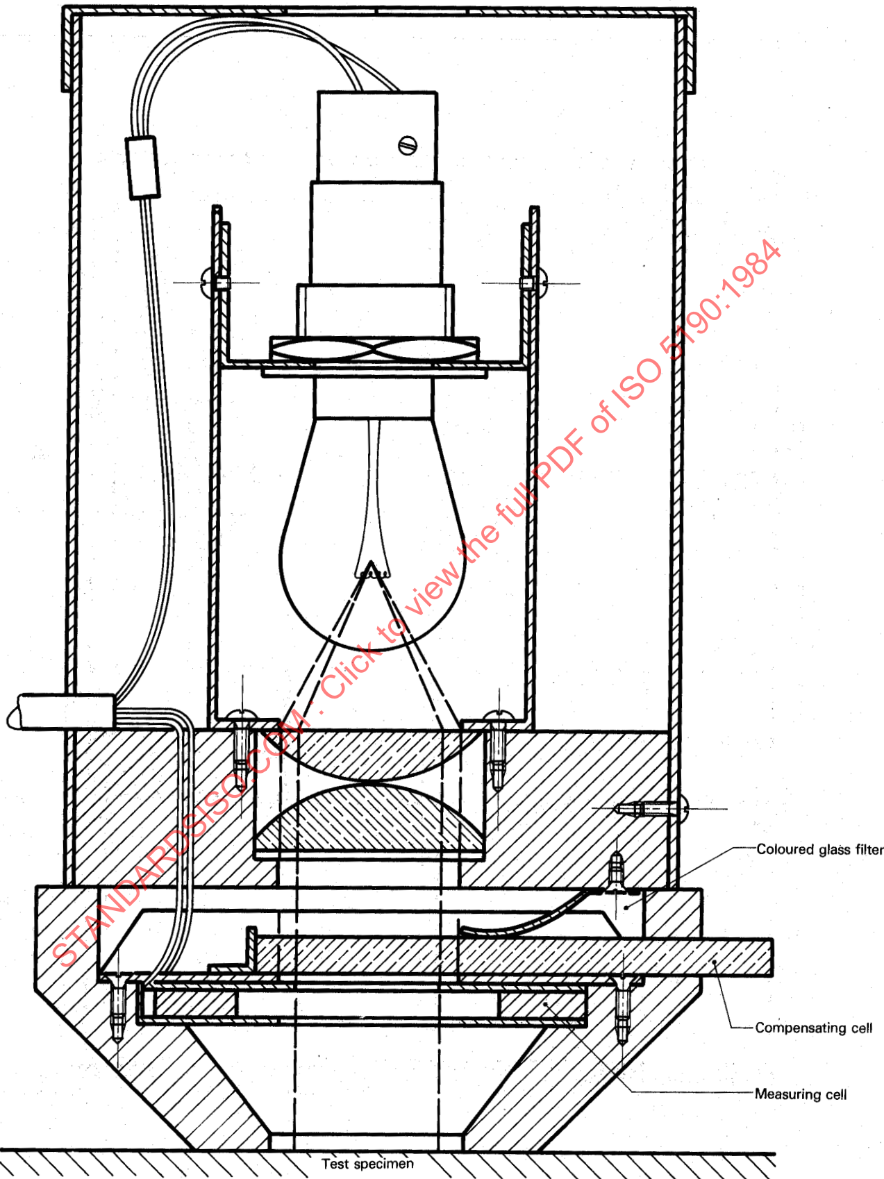
Figure 2 — Example of a tester for measurement of diffuse reflectance
