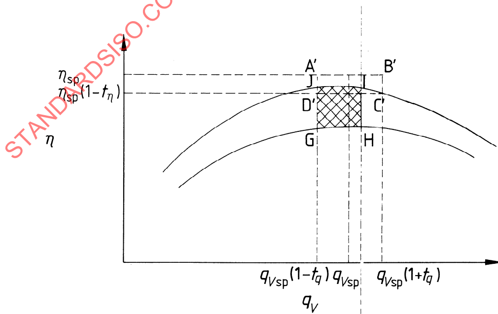
Figure 36 — Graph for comparison of flow rate and efficiency with a specified duty point
