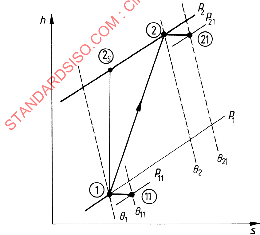
Figure 22 — Enthalpy ( h ) - entropy ( s ) - thermodynamic diagram for water
