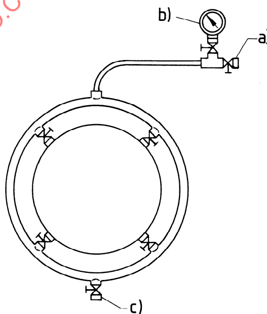
Figure 13 — Pressure tapings connected through ring main to pressure gauge:
