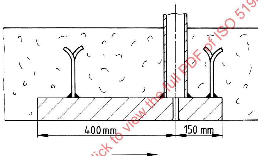
Figure 12 — Example of pressure tapping in concrete wall
