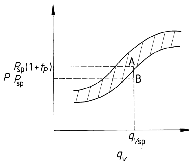
Figure 31 — Graph for comparison of measured power input with that specified at a given flow rate
