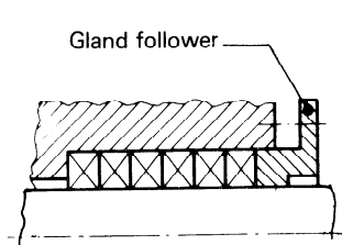
P1 Soft packing
