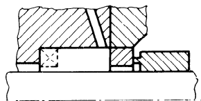
S2 External arrangement
