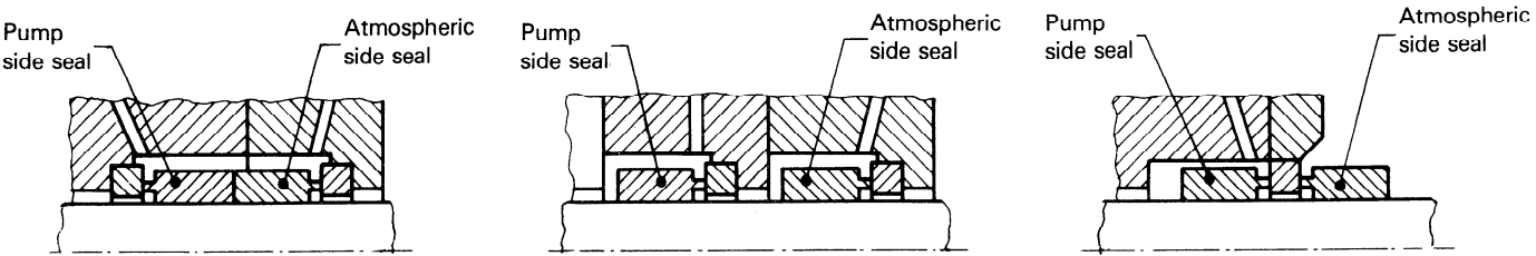
D1 Back-to-back arrangement
