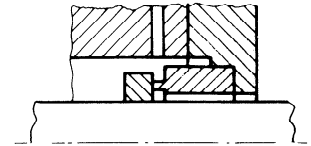
S3 Internal arrangement rotating seal ring (mating ring)
