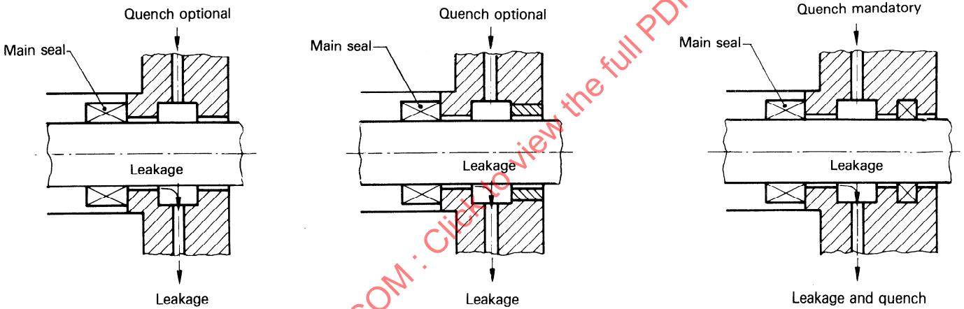
Q1 Main seal without throttle bushing or auxiliary seal
