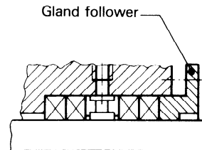
P2 Soft packing with lantern ring (used for injection or circulation of liquid for sealing, buffering, cooling, etc.)
