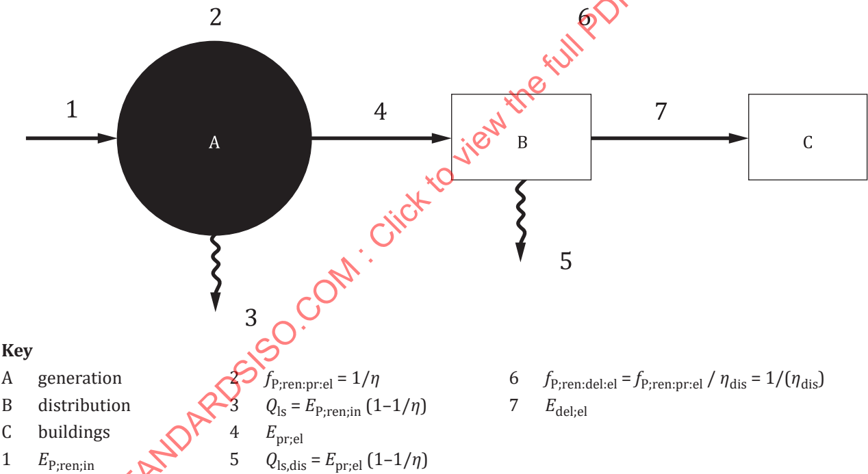
Figure C.1 — Simplified network
