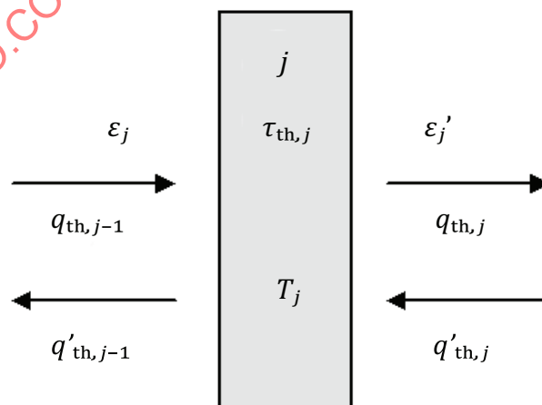
Figure 3 — Schematic presentation of the characteristic data of layer j and the thermal radiative heat flow density
