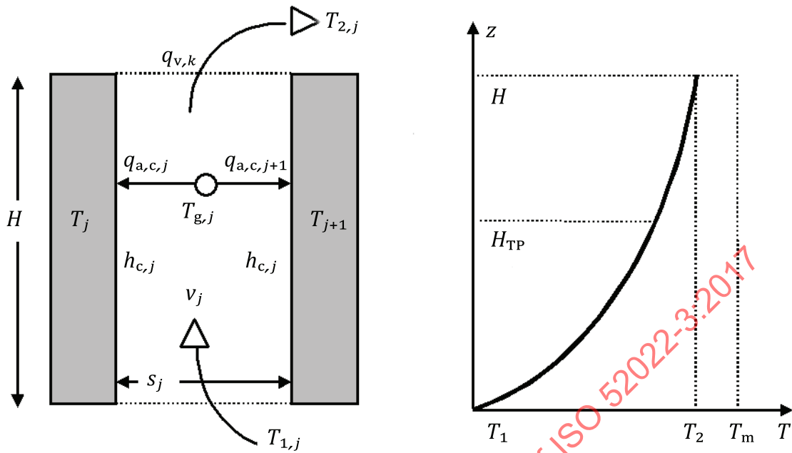
Figure 5 — Schematic presentation of the characteristic data of a ventilated space and the internal temperature profile assuming the incoming air is warmed up
