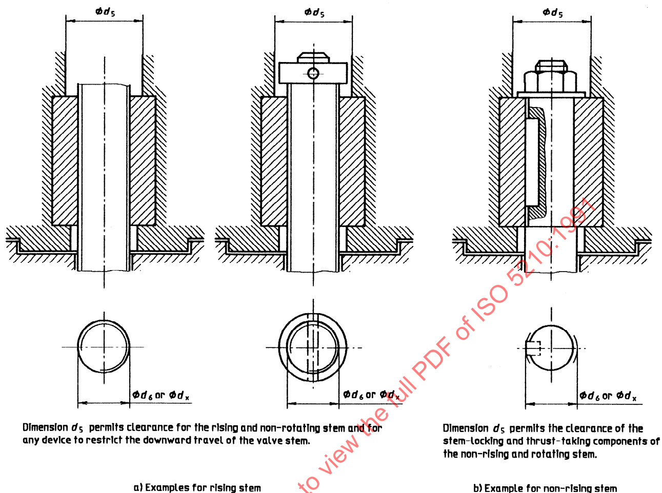
Figure 5 — Driven components, group A
