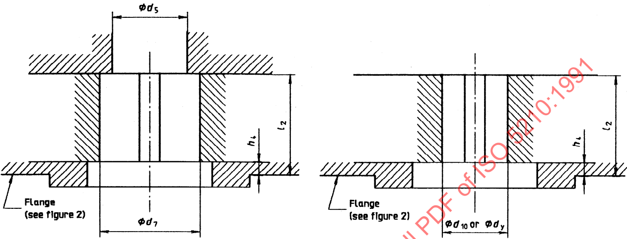
Figure 6 — Driving components, group B
