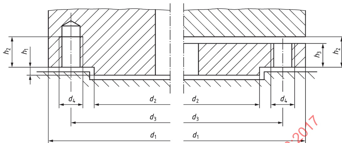
Figure 2 — Flange dimensions
