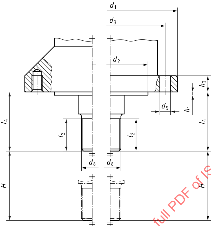
Figure 10 — Dimensions of linear output drive
