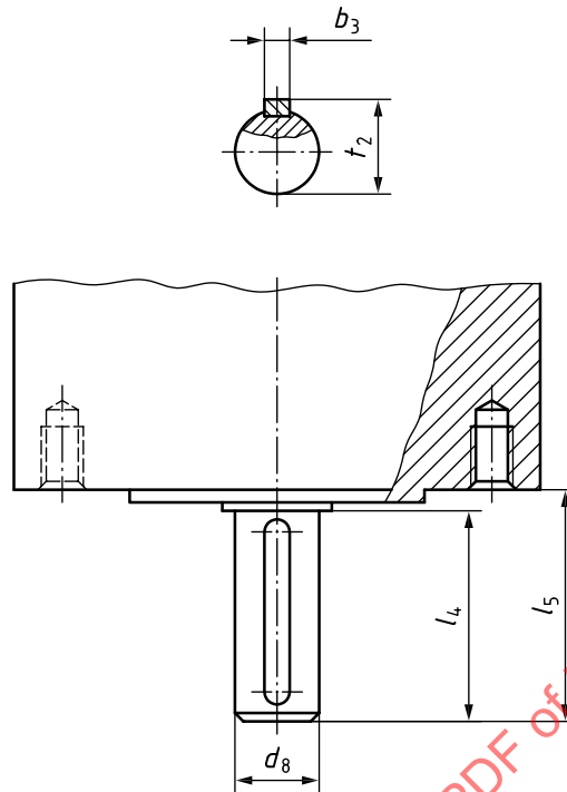
Figure 9 — Driving components, group D
