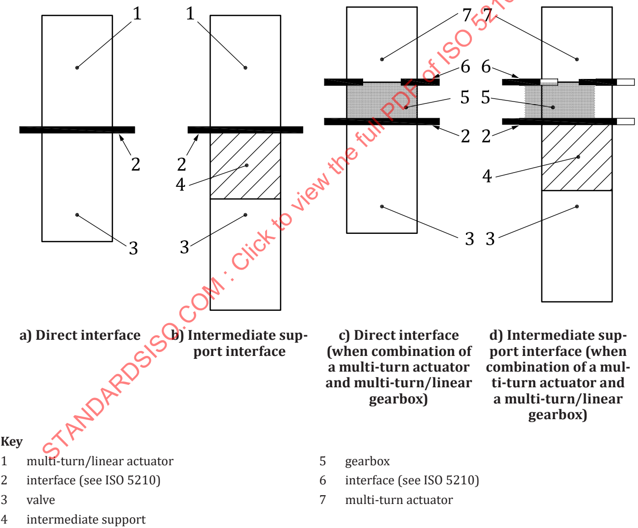
Figure 1 — Interface between multi-turn/linear actuator and valve
