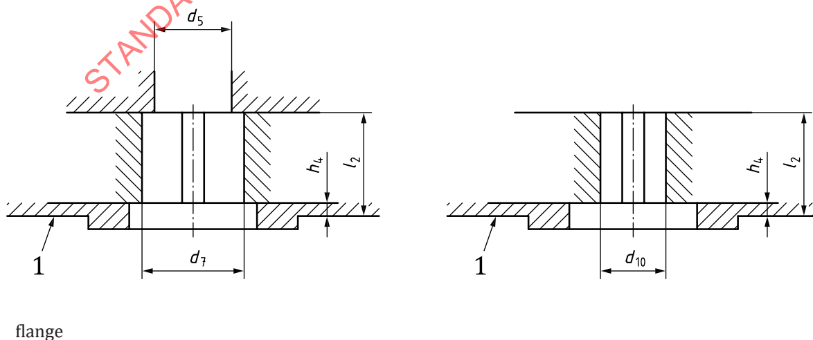
Figure 6 — Driving components, group B
