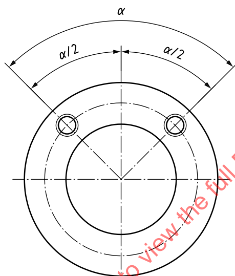
Figure 3 — Positions of the holes for the studs/bolts
