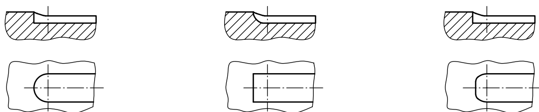
a) Keyway form N1 (groove by end mill) b) Keyway form N2 (groove by disc milling cutter) c) Keyway form N3 (according to specification by valve manufacturer)
