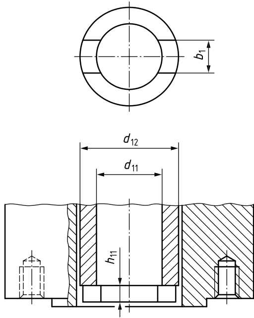
Figure 8 — Driving components, group C
