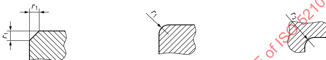
a) Chamfer (according to manufacturer of key) b) Radius (according to manufacturer of key) c) Radius at base of groove for shaft and hub
