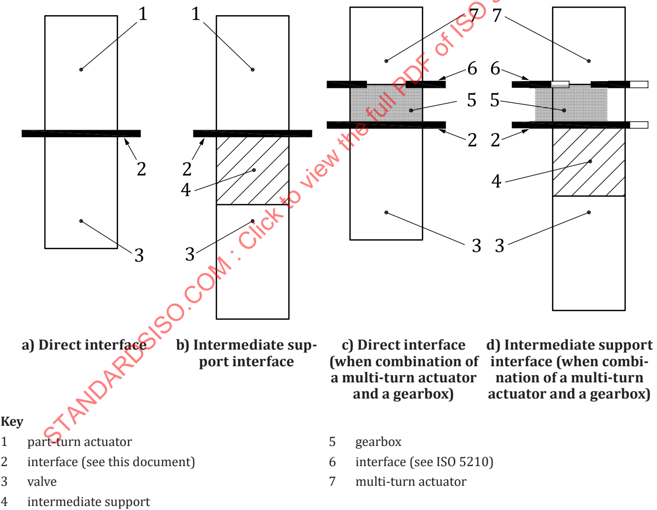
Figure 1 — Interface between part-turn actuator and valve
