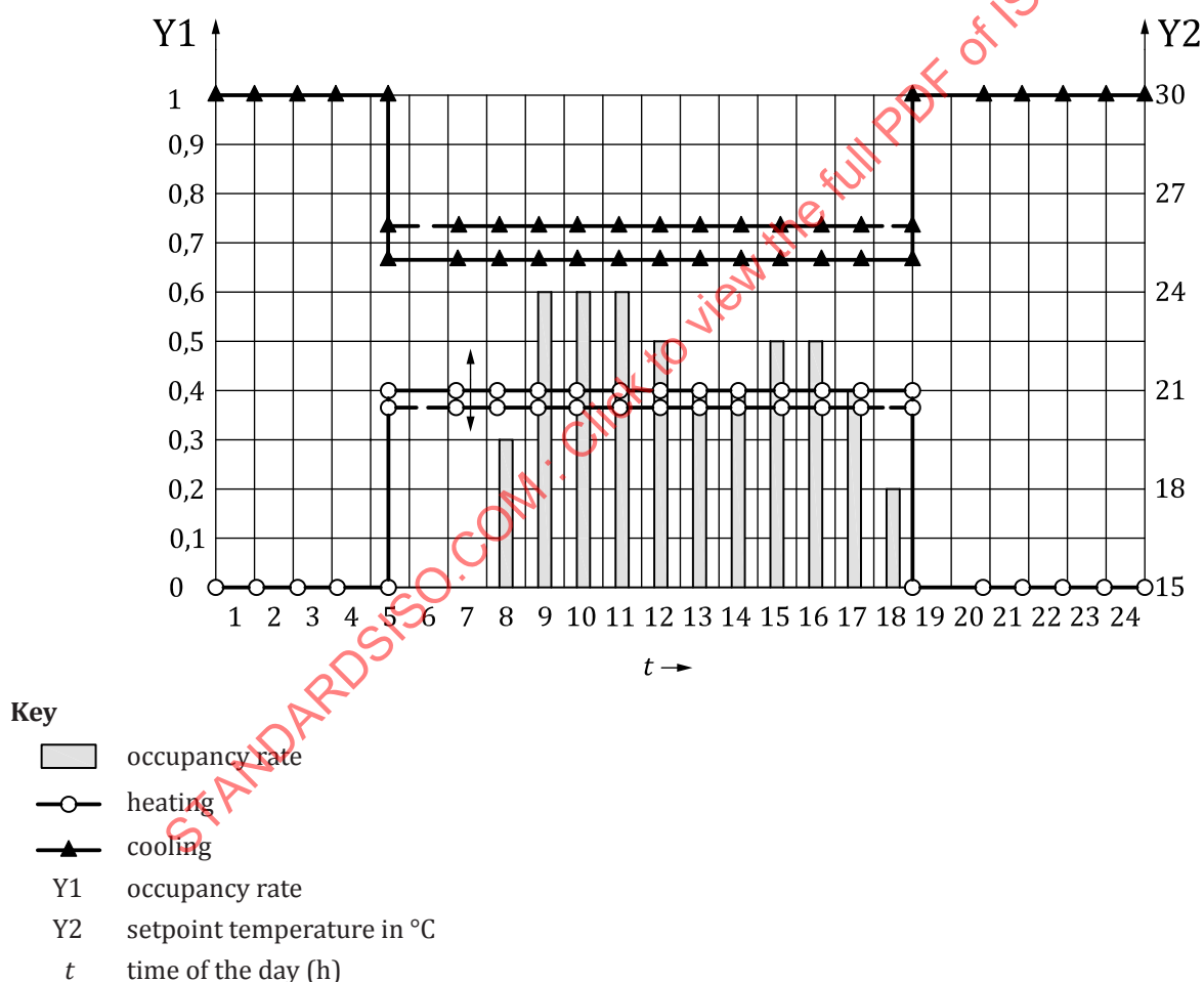
Figure 2 — Adaption of setpoint shifting
