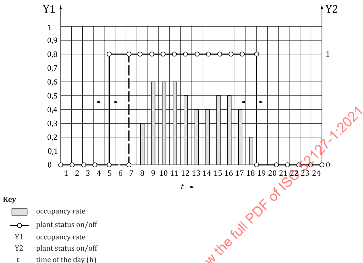
Figure 3 — Adaption of run time
