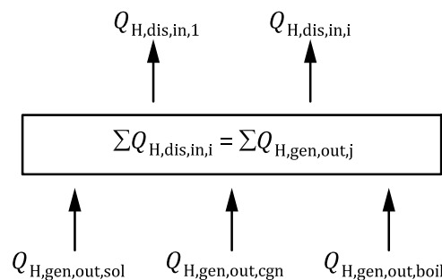
Figure 4 — Example of load splitting among generation sub-systems
