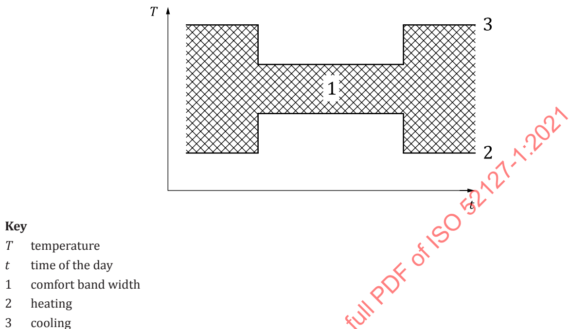
Figure 1 — Typical set point temperature profile
